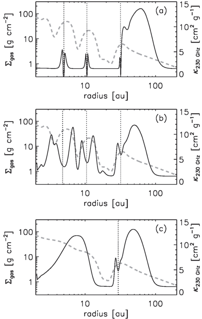
Figure 5. from Diverse Protoplanetary Disk Morphology Produced by a Jupiter-mass Planet null 2018 APJL 864 L26 doi:10.3847/2041-8213/aadd51 https://dx.doi.org/10.3847/2041-8213/aadd51 © 2018. The American Astronomical Society. All rights reserved.
