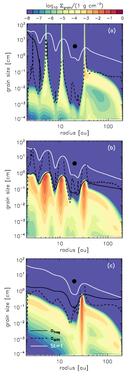
Figure 4. from Diverse Protoplanetary Disk Morphology Produced by a Jupiter-mass Planet null 2018 APJL 864 L26 doi:10.3847/2041-8213/aadd51 https://dx.doi.org/10.3847/2041-8213/aadd51 © 2018. The American Astronomical Society. All rights reserved.
