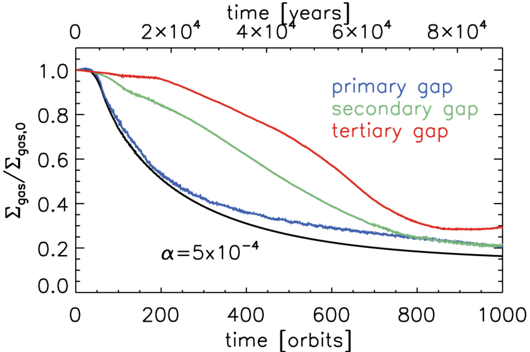
Figure 3. from Diverse Protoplanetary Disk Morphology Produced by a Jupiter-mass Planet null 2018 APJL 864 L26 doi:10.3847/2041-8213/aadd51 https://dx.doi.org/10.3847/2041-8213/aadd51 © 2018. The American Astronomical Society. All rights reserved.
