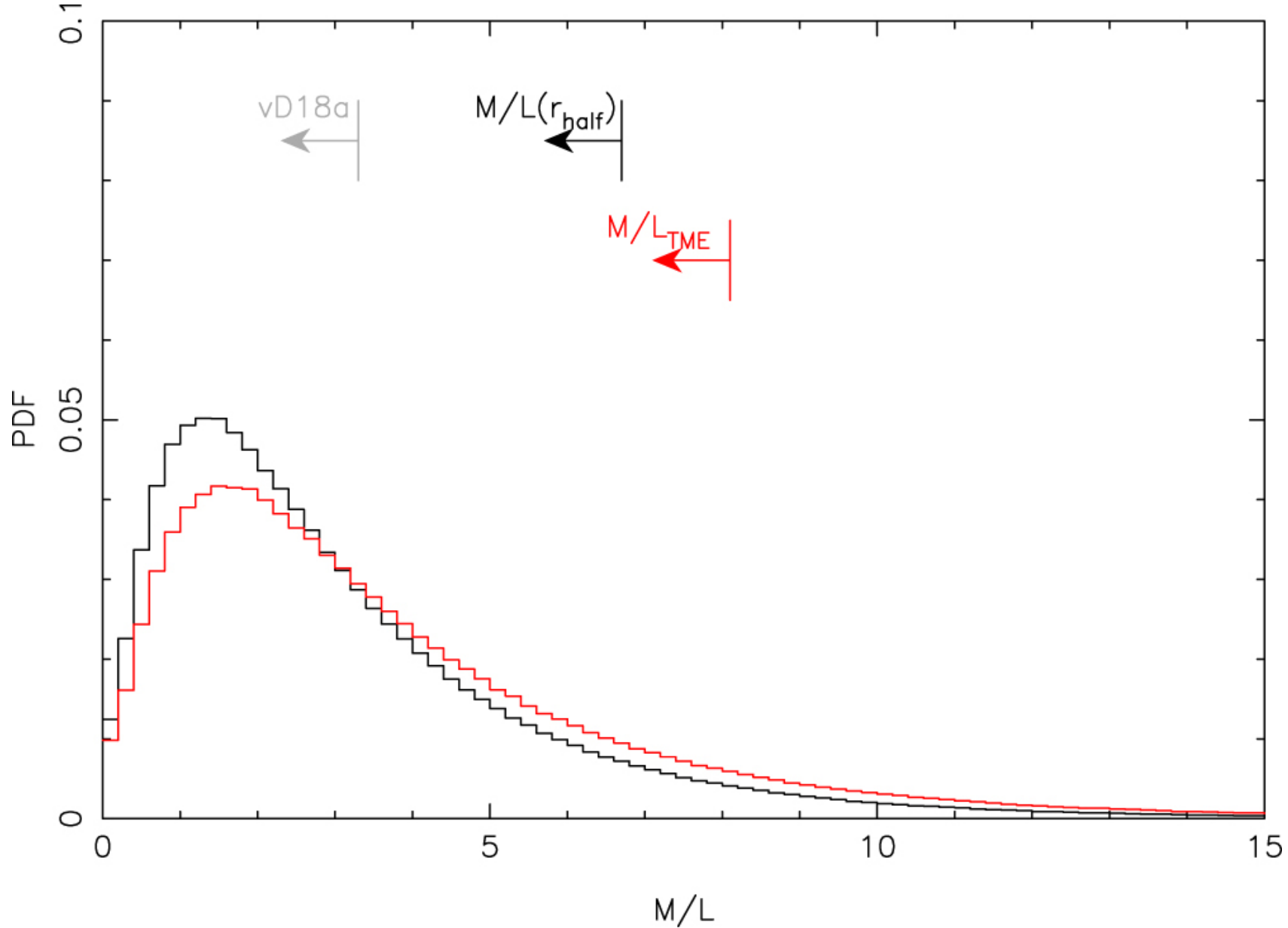
Figure 3. from Current Velocity Data on Dwarf Galaxy NGC 1052-DF2 do not Constrain it to Lack Dark Matter null 2018 APJL 859 L5 doi:10.3847/2041-8213/aac216 https://dx.doi.org/10.3847/2041-8213/aac216 © 2018. The American Astronomical Society. All rights reserved.
