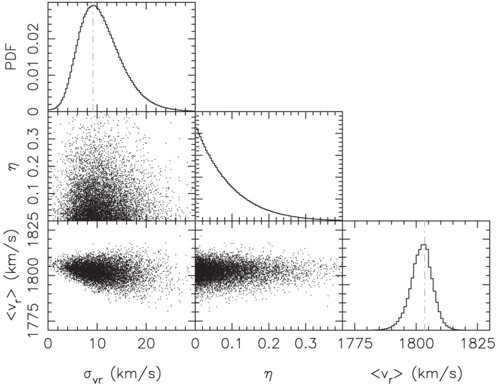
Figure 2. from Current Velocity Data on Dwarf Galaxy NGC 1052-DF2 do not Constrain it to Lack Dark Matter null 2018 APJL 859 L5 doi:10.3847/2041-8213/aac216 https://dx.doi.org/10.3847/2041-8213/aac216 © 2018. The American Astronomical Society. All rights reserved.
