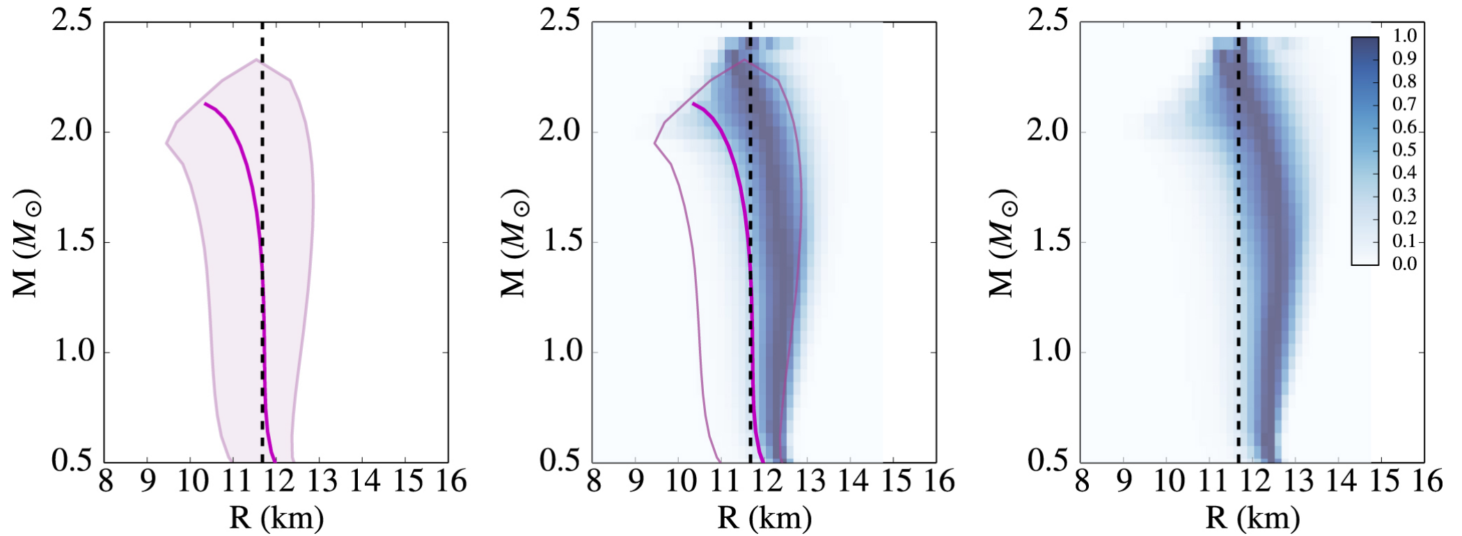
Figure 3. from Tidal Deformability from GW170817 as a Direct Probe of the Neutron Star Radius null 2018 APJL 857 L23 doi:10.3847/2041-8213/aabcbf https://dx.doi.org/10.3847/2041-8213/aabcbf © 2018. The American Astronomical Society. All rights reserved.
