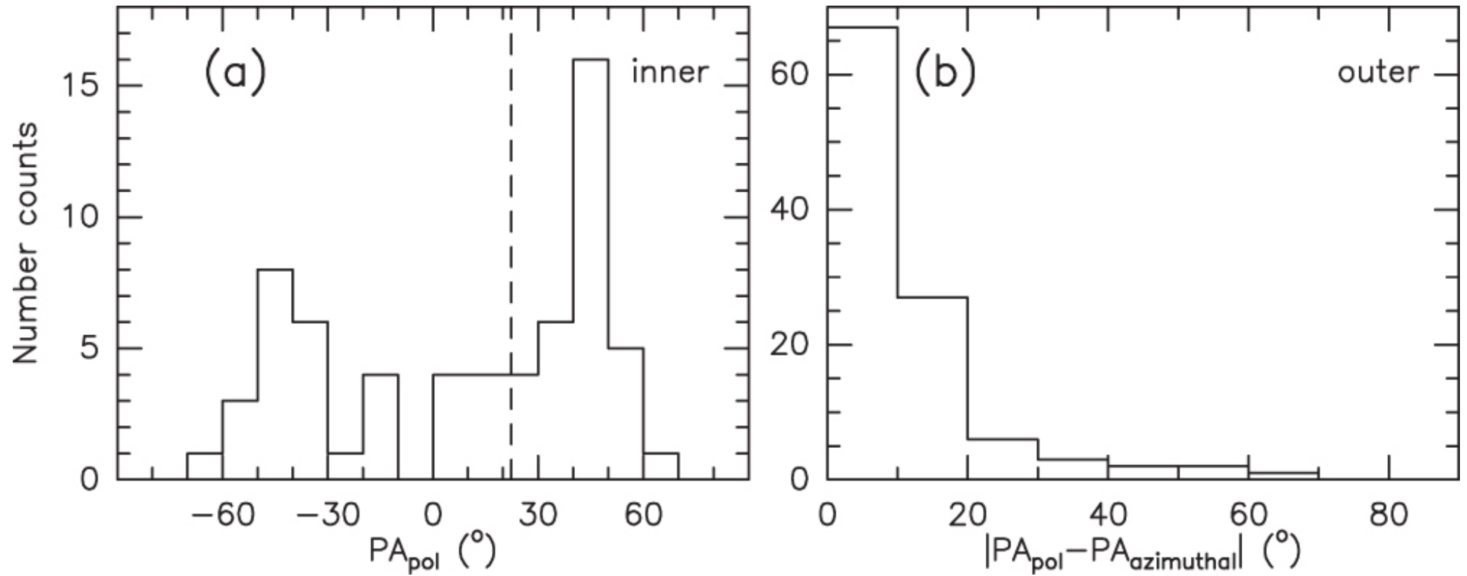
Figure 4. from Resolving the Polarized Dust Emission of the Disk around the Massive Star Powering the HH 80–81 Radio Jet null 2018 APJL 856 L27 doi:10.3847/2041-8213/aab76b https://dx.doi.org/10.3847/2041-8213/aab76b © 2018. The American Astronomical Society. All rights reserved.
