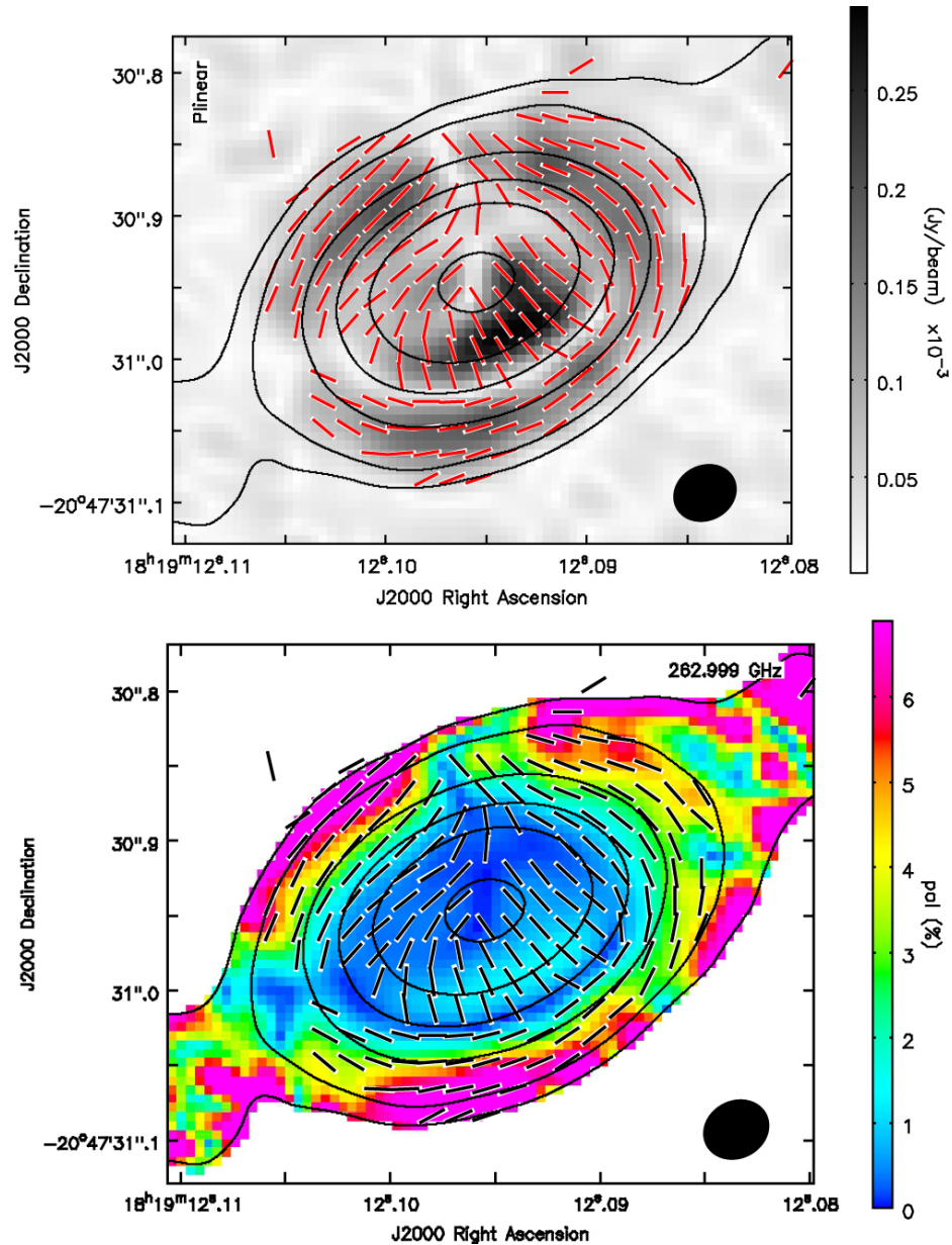
Figure 3. from Resolving the Polarized Dust Emission of the Disk around the Massive Star Powering the HH 80–81 Radio Jet null 2018 APJL 856 L27 doi:10.3847/2041-8213/aab76b https://dx.doi.org/10.3847/2041-8213/aab76b © 2018. The American Astronomical Society. All rights reserved.
