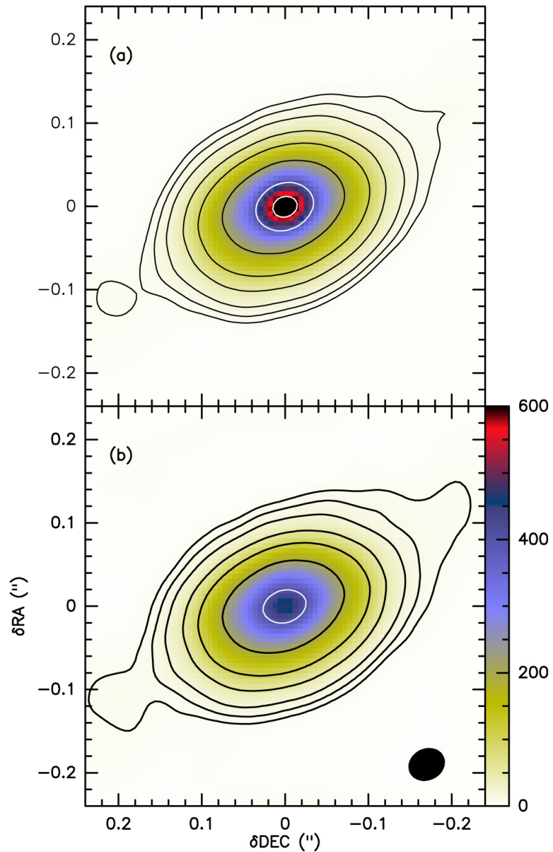
Figure 1. from Resolving the Polarized Dust Emission of the Disk around the Massive Star Powering the HH 80–81 Radio Jet null 2018 APJL 856 L27 doi:10.3847/2041-8213/aab76b https://dx.doi.org/10.3847/2041-8213/aab76b © 2018. The American Astronomical Society. All rights reserved.
