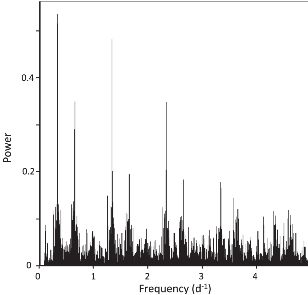
Figure 1. from The Binary Dwarf Carbon Star SDSS J125017.90+252427.6 null 2018 APJL 856 L2 doi:10.3847/2041-8213/aab42a https://dx.doi.org/10.3847/2041-8213/aab42a © 2018. The American Astronomical Society. All rights reserved.
