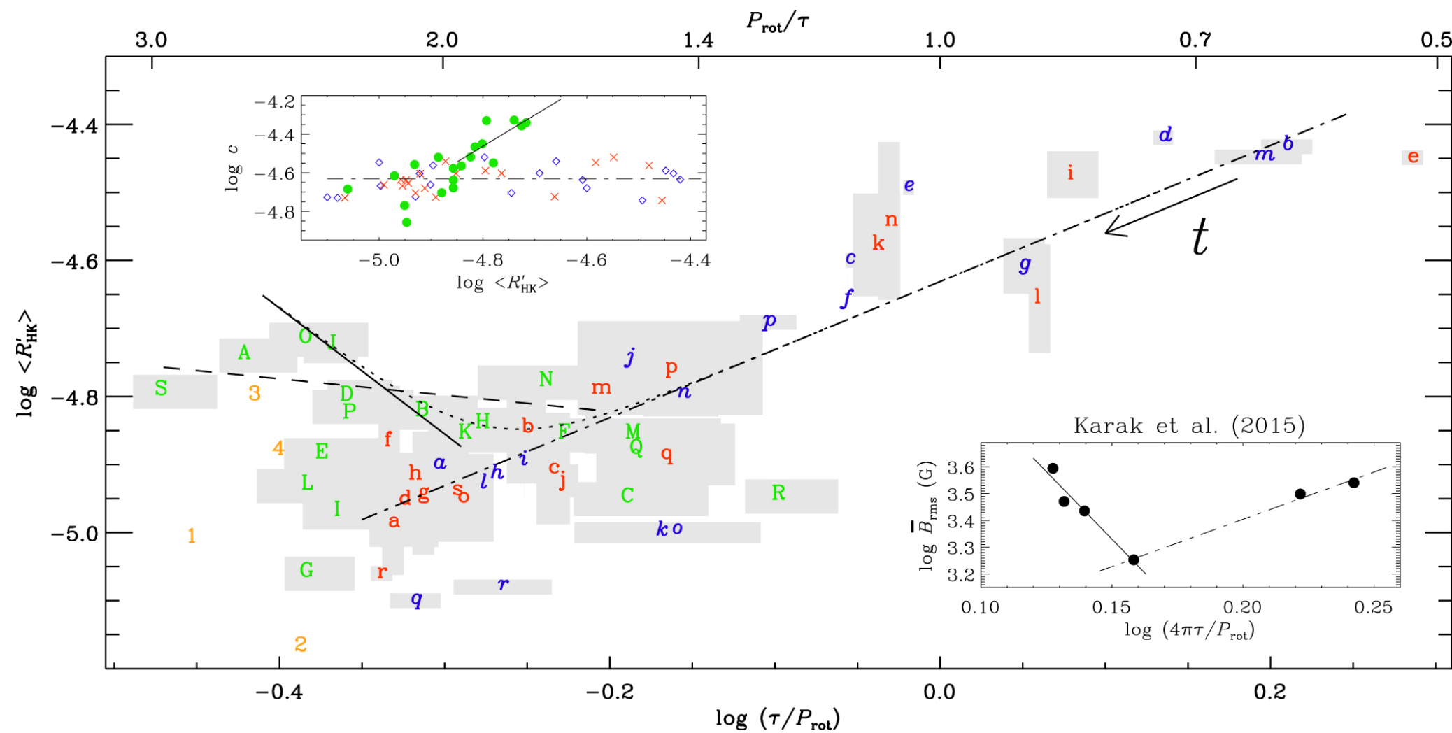
Figure 1. from Enhanced Stellar Activity for Slow Antisolar Differential Rotation? null 2018 APJL 855 L22 doi:10.3847/2041-8213/aab20a https://dx.doi.org/10.3847/2041-8213/aab20a © 2018. The American Astronomical Society. All rights reserved.
