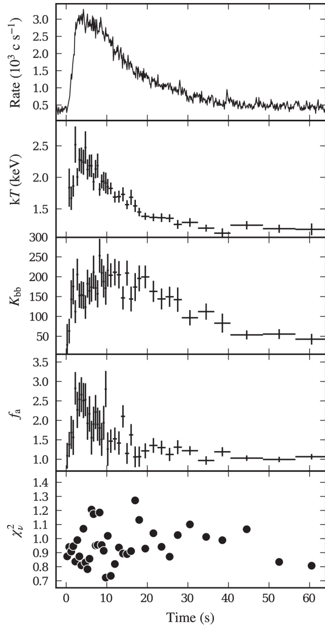
Figure 4. from NICER Observes the Effects of an X-Ray Burst on the Accretion Environment in Aql X-1 null 2018 APJL 855 L4 doi:10.3847/2041-8213/aab104 https://dx.doi.org/10.3847/2041-8213/aab104 © 2018. The American Astronomical Society. All rights reserved.
