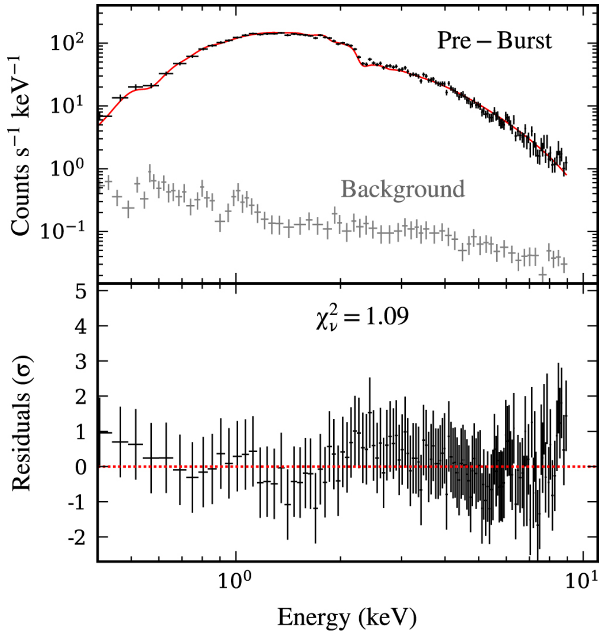
Figure 2. from NICER Observes the Effects of an X-Ray Burst on the Accretion Environment in Aql X-1 null 2018 APJL 855 L4 doi:10.3847/2041-8213/aab104 https://dx.doi.org/10.3847/2041-8213/aab104 © 2018. The American Astronomical Society. All rights reserved.
