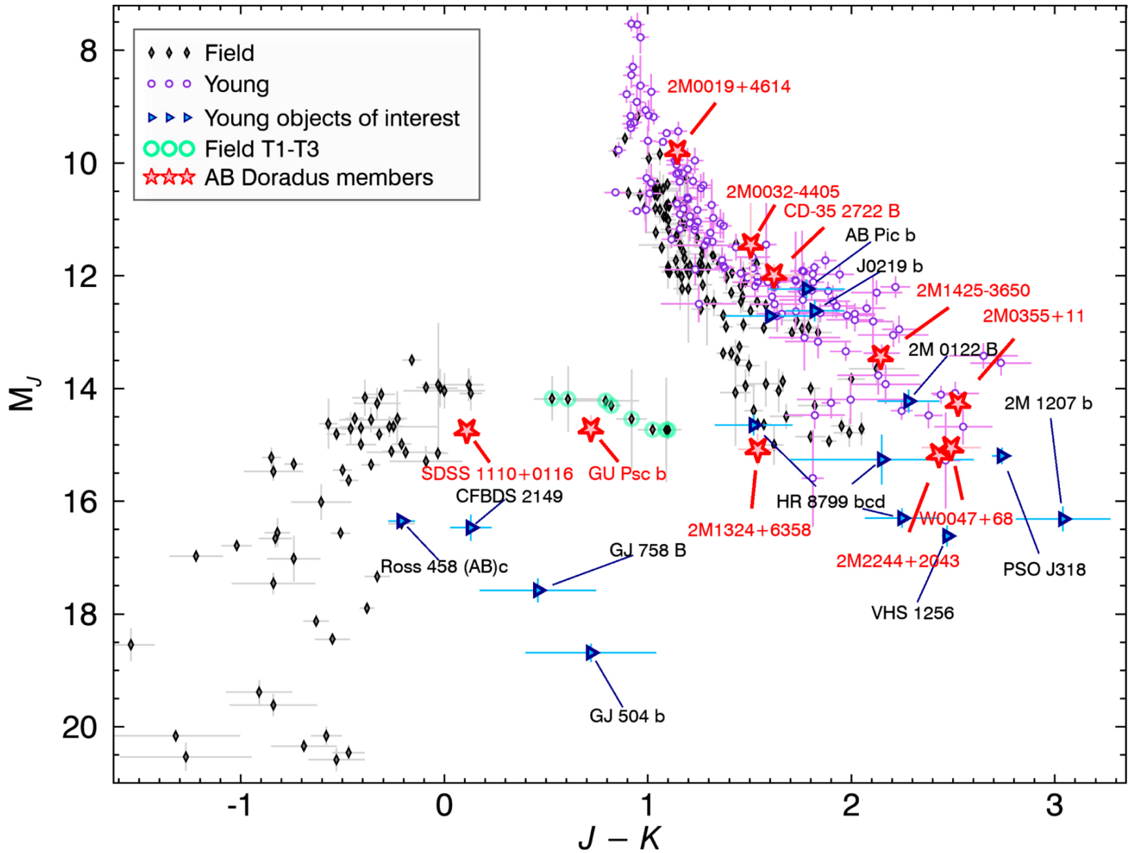
Figure 4. from 2MASS J13243553+6358281 Is an Early T-type Planetary-mass Object in the AB Doradus Moving Group null 2018 APJL 854 L27 doi:10.3847/2041-8213/aaacfd https://dx.doi.org/10.3847/2041-8213/aaacfd © 2018. The American Astronomical Society. All rights reserved.
