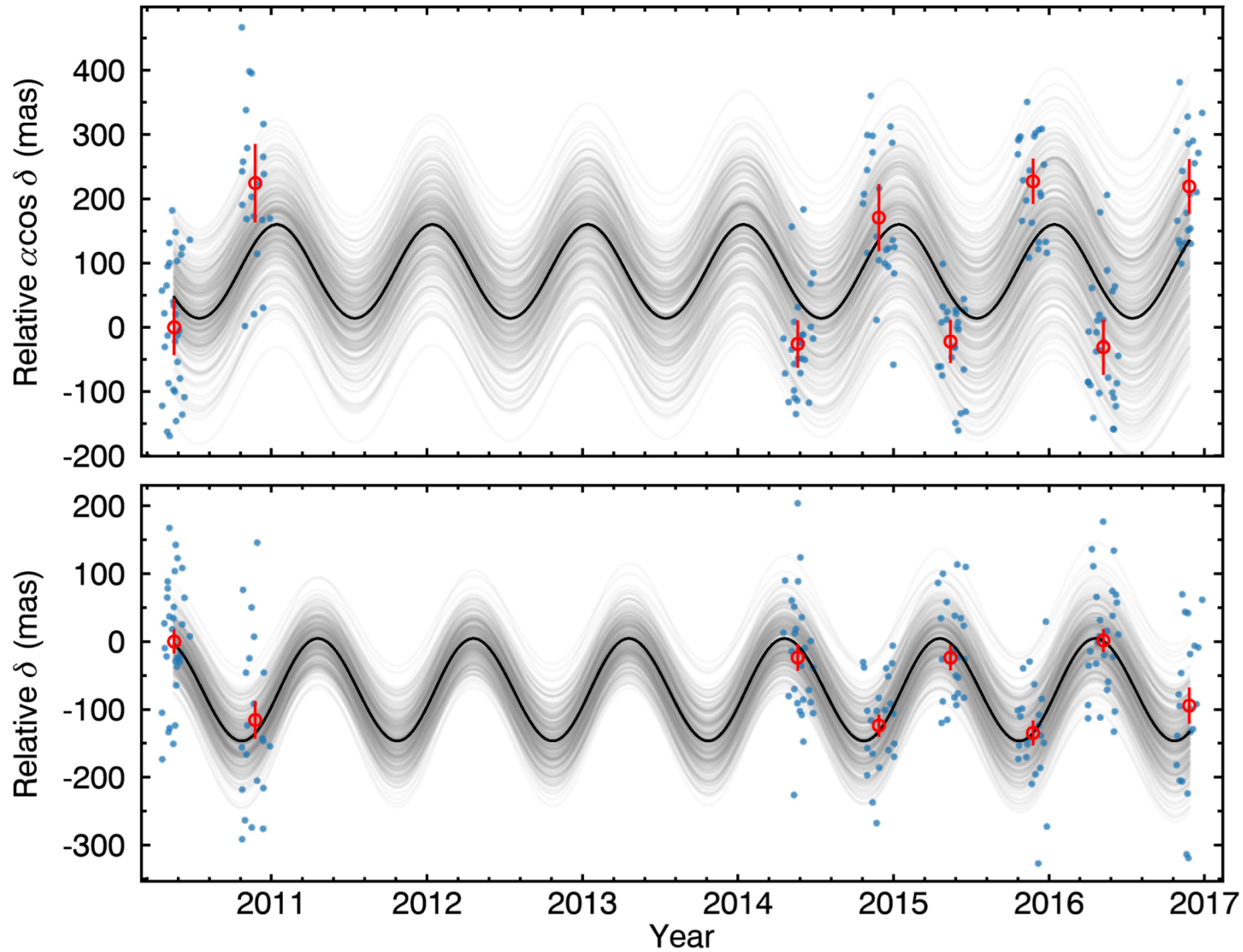
Figure 3. from 2MASS J13243553+6358281 Is an Early T-type Planetary-mass Object in the AB Doradus Moving Group null 2018 APJL 854 L27 doi:10.3847/2041-8213/aaacfd https://dx.doi.org/10.3847/2041-8213/aaacfd © 2018. The American Astronomical Society. All rights reserved.
