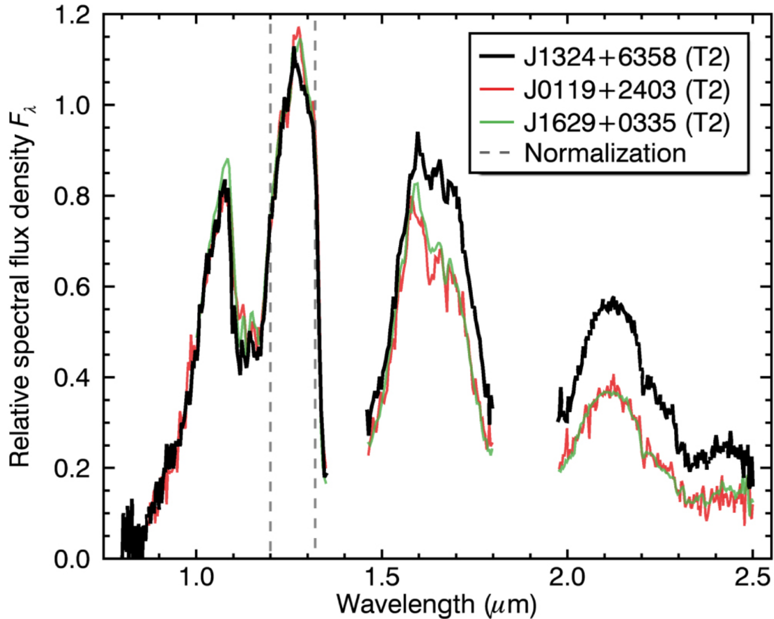
Figure 1. from 2MASS J13243553+6358281 Is an Early T-type Planetary-mass Object in the AB Doradus Moving Group null 2018 APJL 854 L27 doi:10.3847/2041-8213/aaacfd https://dx.doi.org/10.3847/2041-8213/aaacfd © 2018. The American Astronomical Society. All rights reserved.
