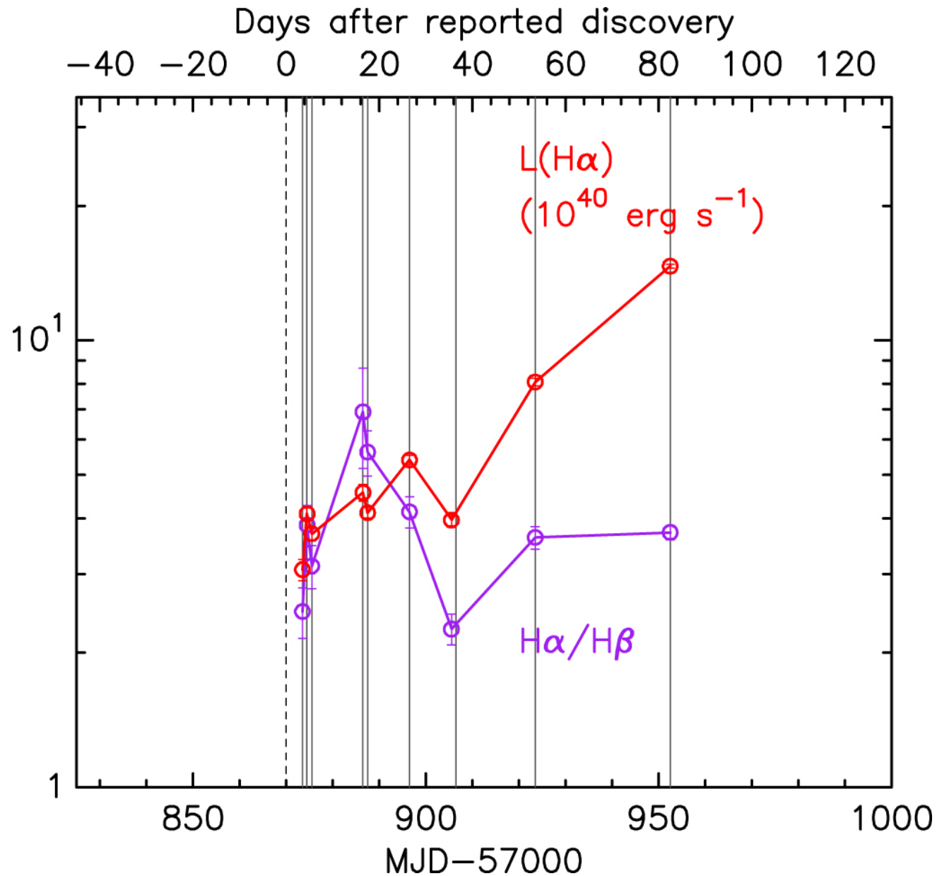
Figure 5. from SN 2017dio: A Type-Ic Supernova Exploding in a Hydrogen-rich Circumstellar Medium null 2018 APJL 854 L14 doi:10.3847/2041-8213/aaaa1a https://dx.doi.org/10.3847/2041-8213/aaaa1a © 2018. The American Astronomical Society. All rights reserved.
