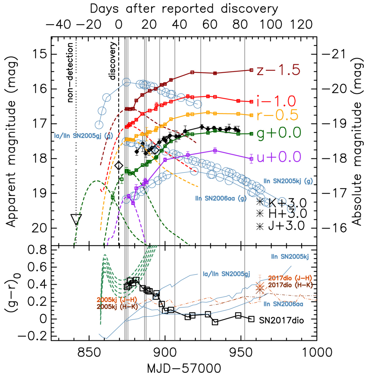
Figure 2. from SN 2017dio: A Type-Ic Supernova Exploding in a Hydrogen-rich Circumstellar Medium null 2018 APJL 854 L14 doi:10.3847/2041-8213/aaaa1a https://dx.doi.org/10.3847/2041-8213/aaaa1a
