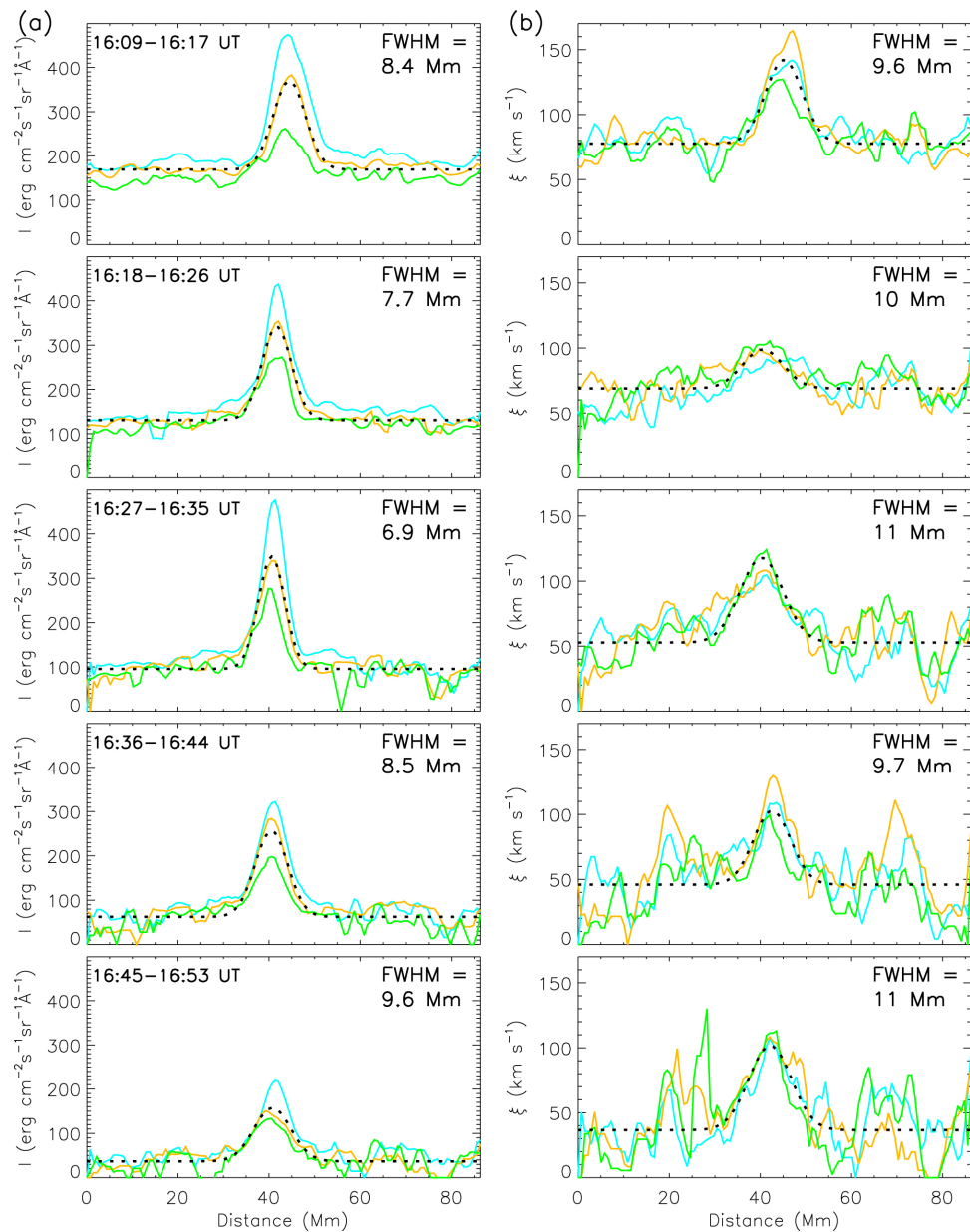
Figure 5. from Spectroscopic Observations of a Current Sheet in a Solar Flare null 2018 APJL 853 L15 doi:10.3847/2041-8213/aaa6c0 https://dx.doi.org/10.3847/2041-8213/aaa6c0 © 2018. The American Astronomical Society. All rights reserved.
