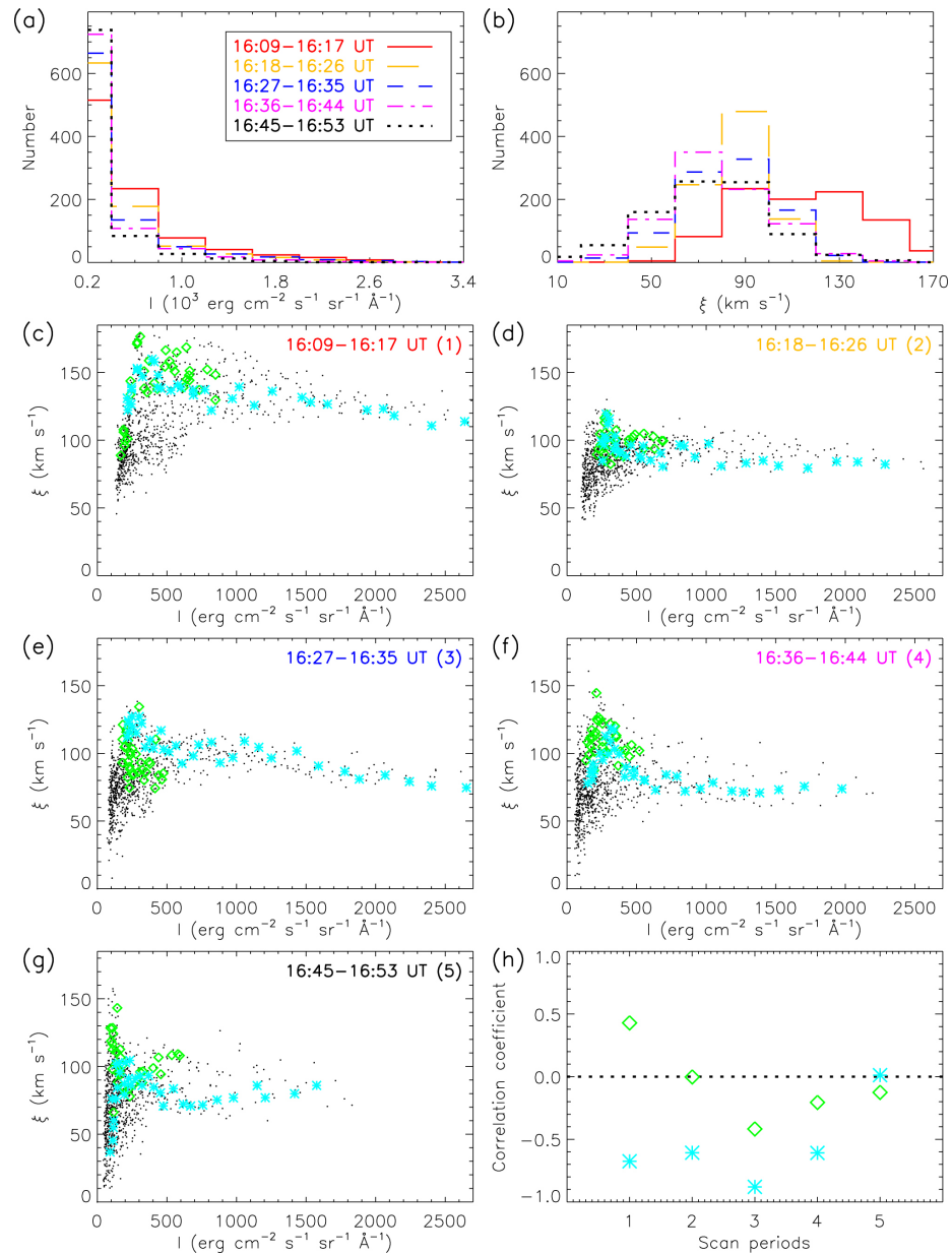
Figure 4. from Spectroscopic Observations of a Current Sheet in a Solar Flare null 2018 APJL 853 L15 doi:10.3847/2041-8213/aaa6c0 https://dx.doi.org/10.3847/2041-8213/aaa6c0
