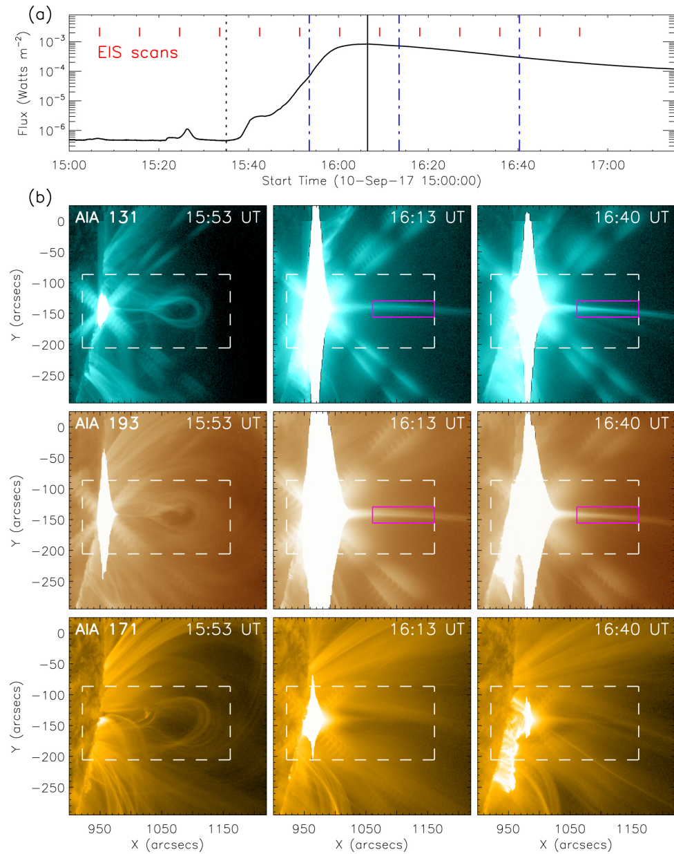
Figure 1. from Spectroscopic Observations of a Current Sheet in a Solar Flare null 2018 APJL 853 L15 doi:10.3847/2041-8213/aaa6c0 https://dx.doi.org/10.3847/2041-8213/aaa6c0 © 2018. The American Astronomical Society. All rights reserved.
