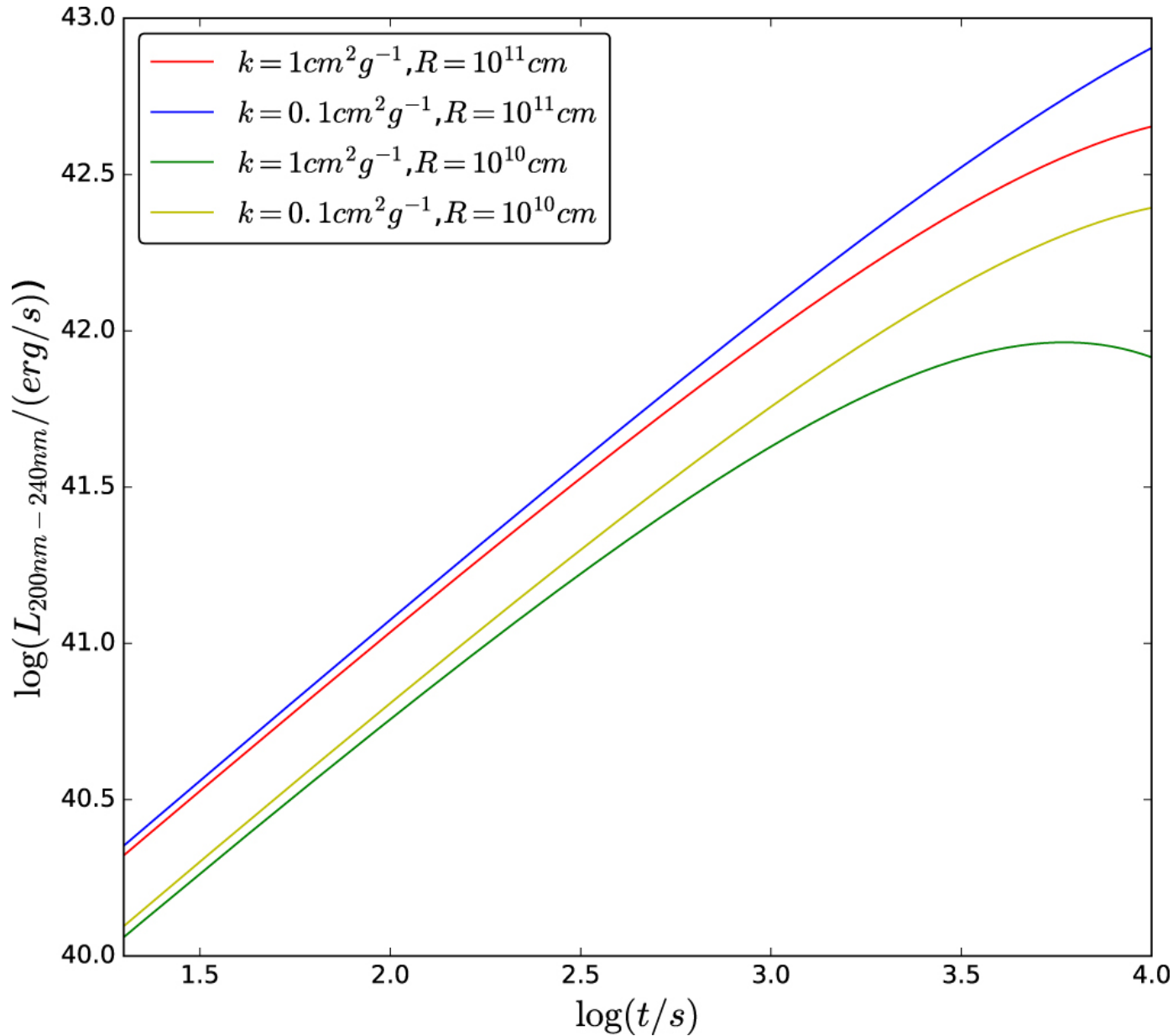
Figure 2. from Early Soft X-Ray to UV Emission from Double Neutron Star Mergers: Implications from the Long-term Observations of GW170817 null 2018 APJL 853 L13 doi:10.3847/2041-8213/aaa5fc https://dx.doi.org/10.3847/2041-8213/aaa5fc © 2018. The American Astronomical Society.
