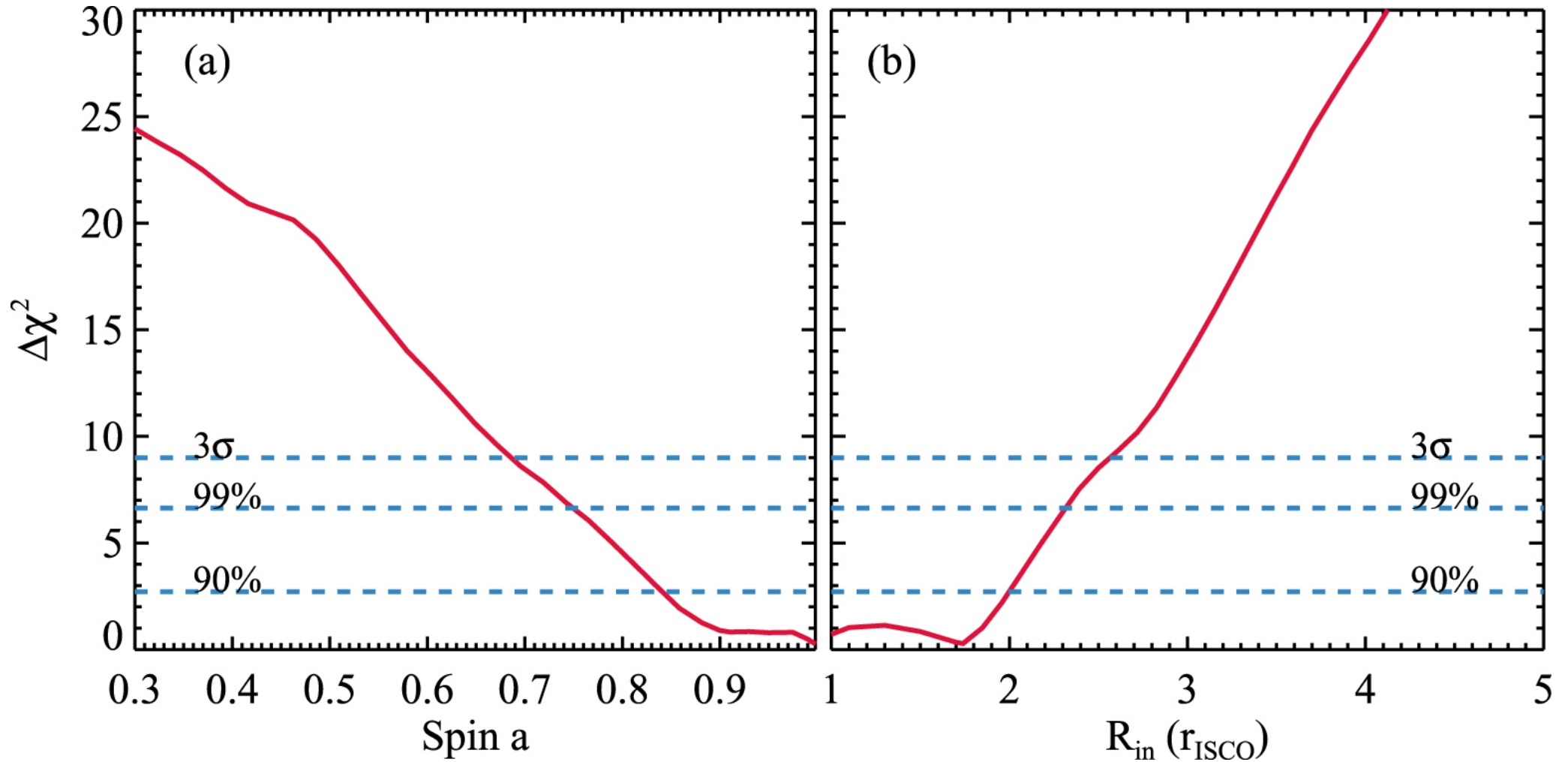
Figure 4. from Reflection Spectra of the Black Hole Binary Candidate MAXI J1535-571 in the Hard State Observed by NuSTAR null 2018 APJL 852 L34 doi:10.3847/2041-8213/aaa4b2 https://dx.doi.org/10.3847/2041-8213/aaa4b2 © 2018. The American Astronomical Society. All rights reserved.
