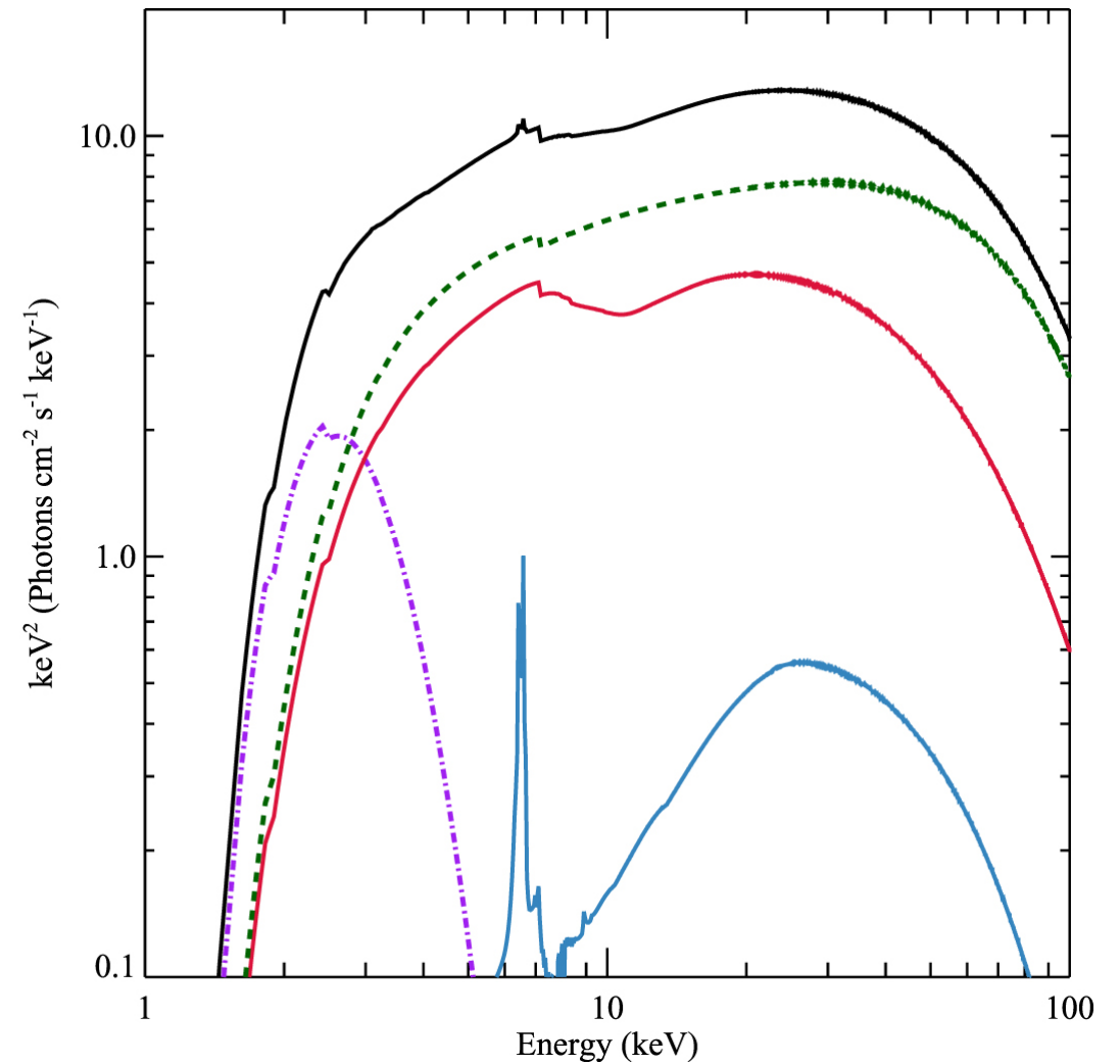
Figure 3. from Reflection Spectra of the Black Hole Binary Candidate MAXI J1535-571 in the Hard State Observed by NuSTAR null 2018 APJL 852 L34 doi:10.3847/2041-8213/aaa4b2 https://dx.doi.org/10.3847/2041-8213/aaa4b2
