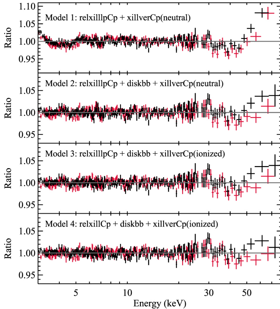
Figure 3. from Reflection Spectra of the Black Hole Binary Candidate MAXI J1535-571 in the Hard State Observed by NuSTAR null 2018 APJL 852 L34 doi:10.3847/2041-8213/aaa4b2 https://dx.doi.org/10.3847/2041-8213/aaa4b2
