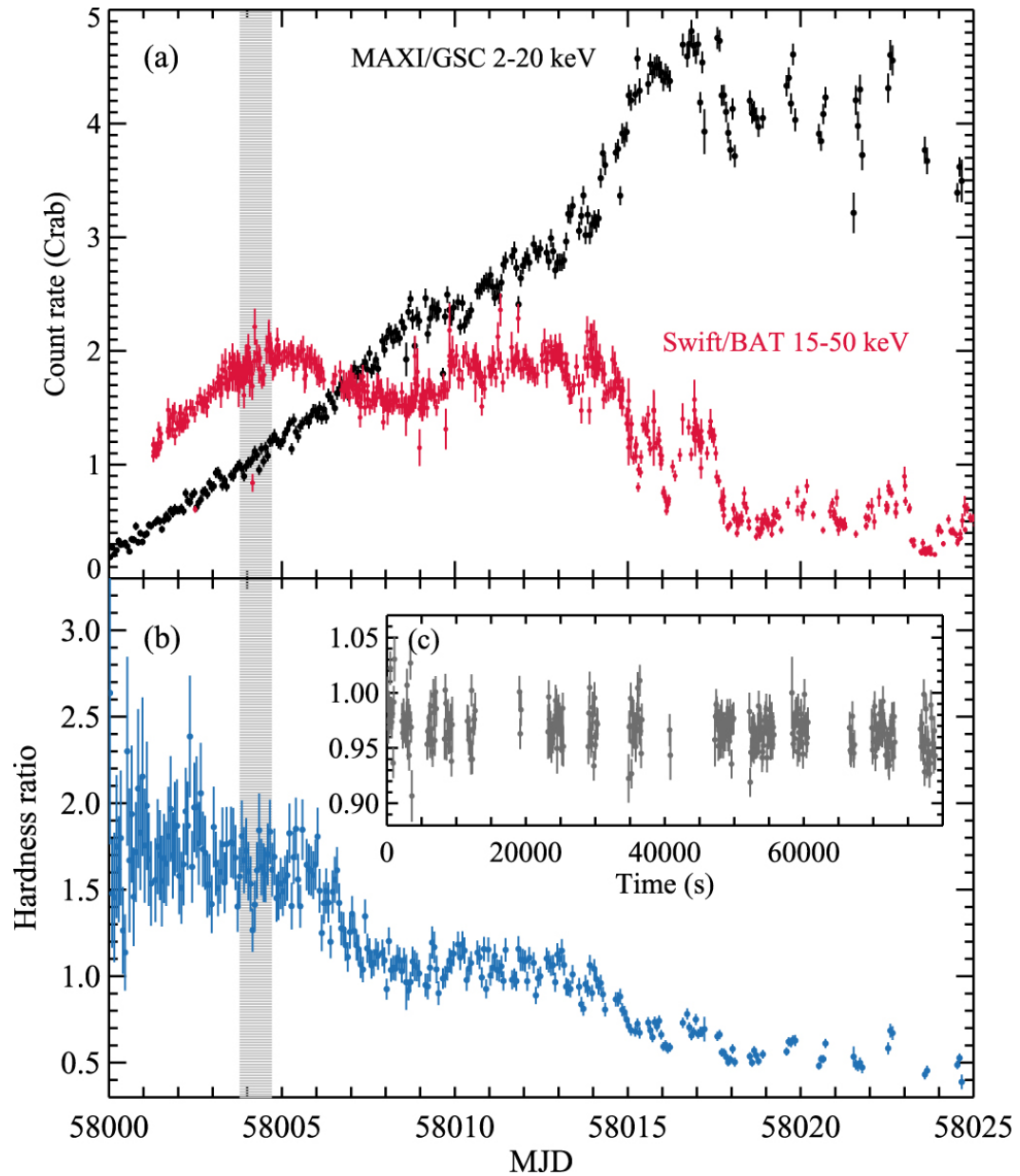
Figure 1. from Reflection Spectra of the Black Hole Binary Candidate MAXI J1535-571 in the Hard State Observed by NuSTAR null 2018 APJL 852 L34 doi:10.3847/2041-8213/aaa4b2 https://dx.doi.org/10.3847/2041-8213/aaa4b2
