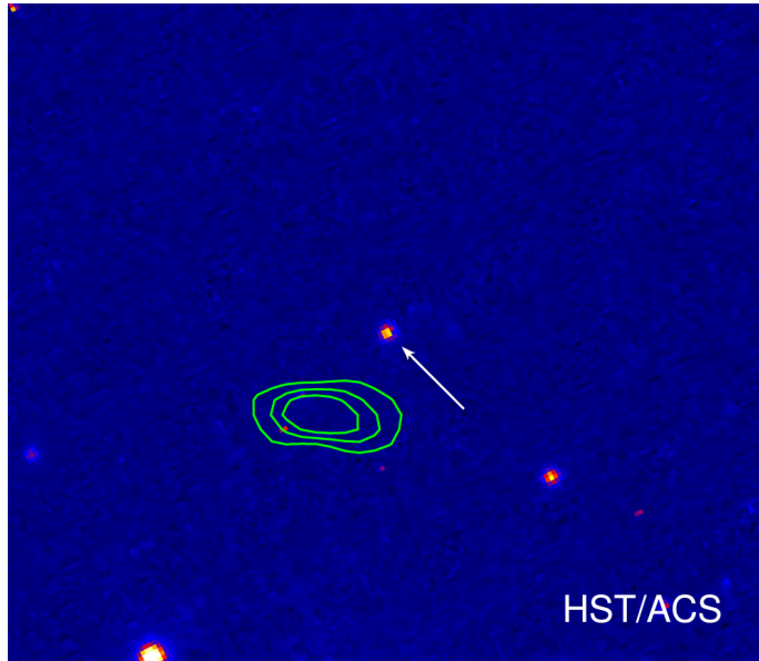
Figure 3. from The First Detection of a Pulsar with ALMA null 2017 APJL 851 L10 doi:10.3847/2041-8213/aa9c3e https://dx.doi.org/10.3847/2041-8213/aa9c3e © 2017. The American Astronomical Society. All rights reserved.
