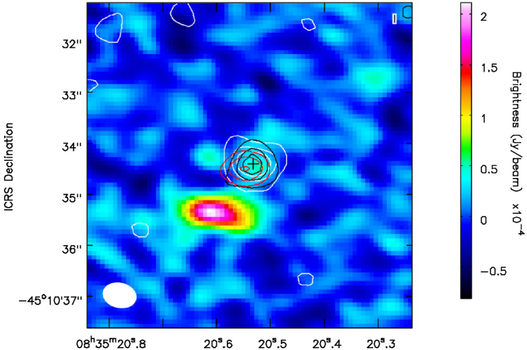
Figure 1. from The First Detection of a Pulsar with ALMA null 2017 APJL 851 L10 doi:10.3847/2041-8213/aa9c3e https://dx.doi.org/10.3847/2041-8213/aa9c3e © 2017. The American Astronomical Society. All rights reserved.
