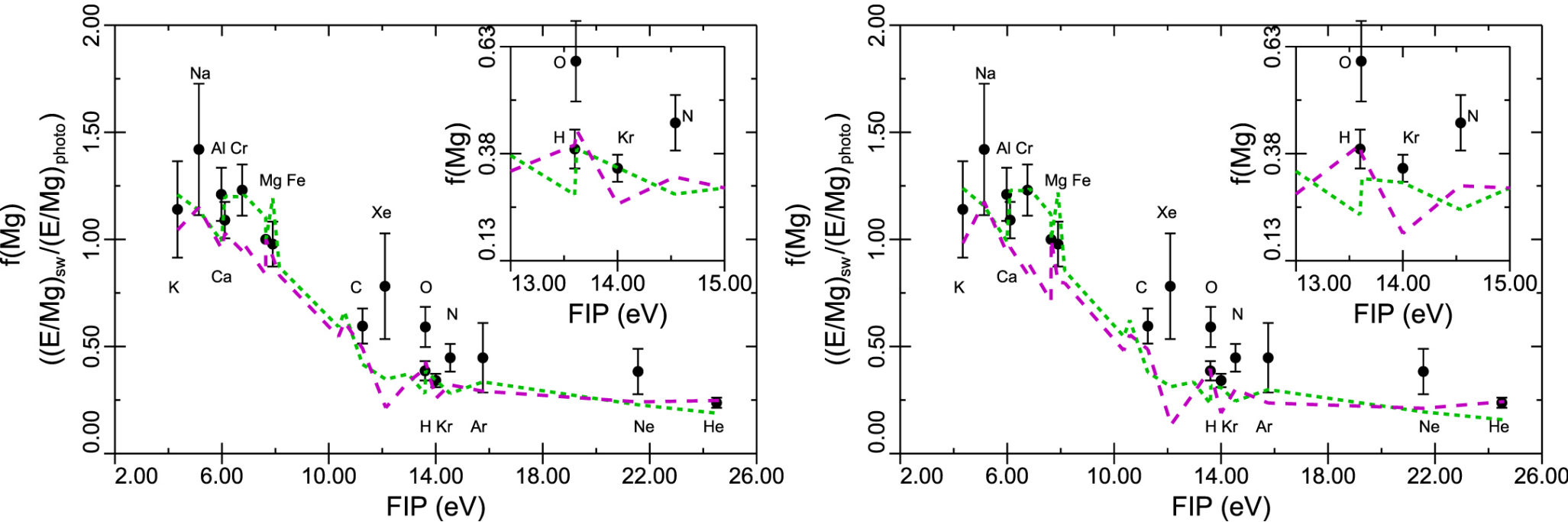
Figure 3. from Determining the Elemental and Isotopic Composition of the Pre-solar Nebula from Genesis Data Analysis: The Case of Oxygen null 2017 APJL 851 L12 doi:10.3847/2041-8213/aa9bf0 https://dx.doi.org/10.3847/2041-8213/aa9bf0 © 2017. The American Astronomical Society. All rights reserved.
