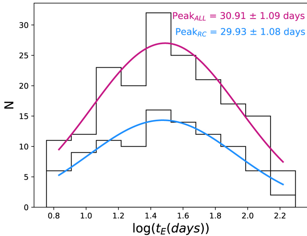
Figure 3. from VVV Survey Microlensing Events in the Galactic Center Region null 2017 APJL 851 L13 doi:10.3847/2041-8213/aa9b29 https://dx.doi.org/10.3847/2041-8213/aa9b29 © 2017. The American Astronomical Society. All rights reserved.
