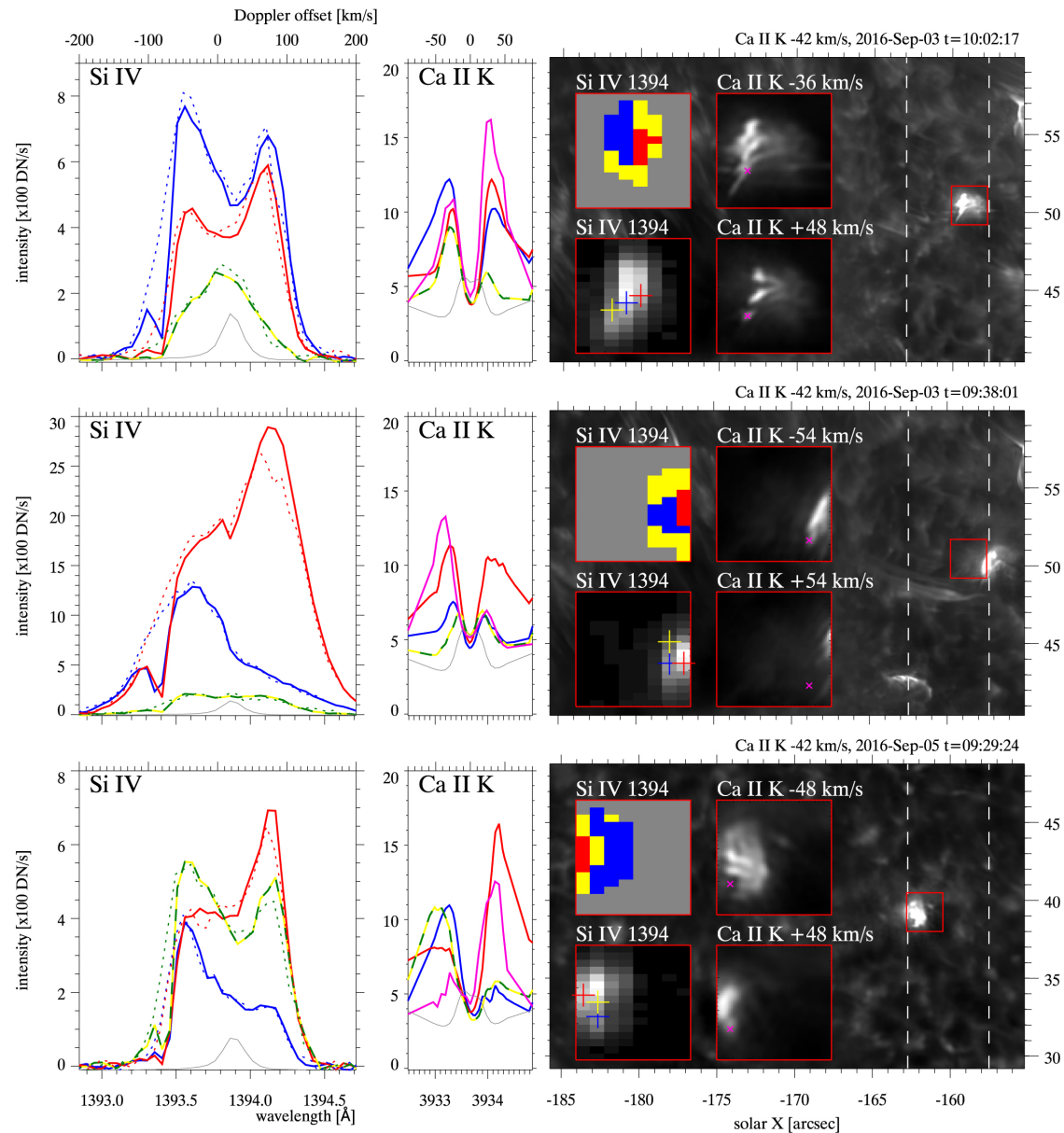
Figure 3. from Intermittent Reconnection and Plasmoids in UV Bursts in the Low Solar Atmosphere null 2017 APJL 851 L6 doi:10.3847/2041-8213/aa99dd https://dx.doi.org/10.3847/2041-8213/aa99dd © 2017. The American Astronomical Society. All rights reserved.
