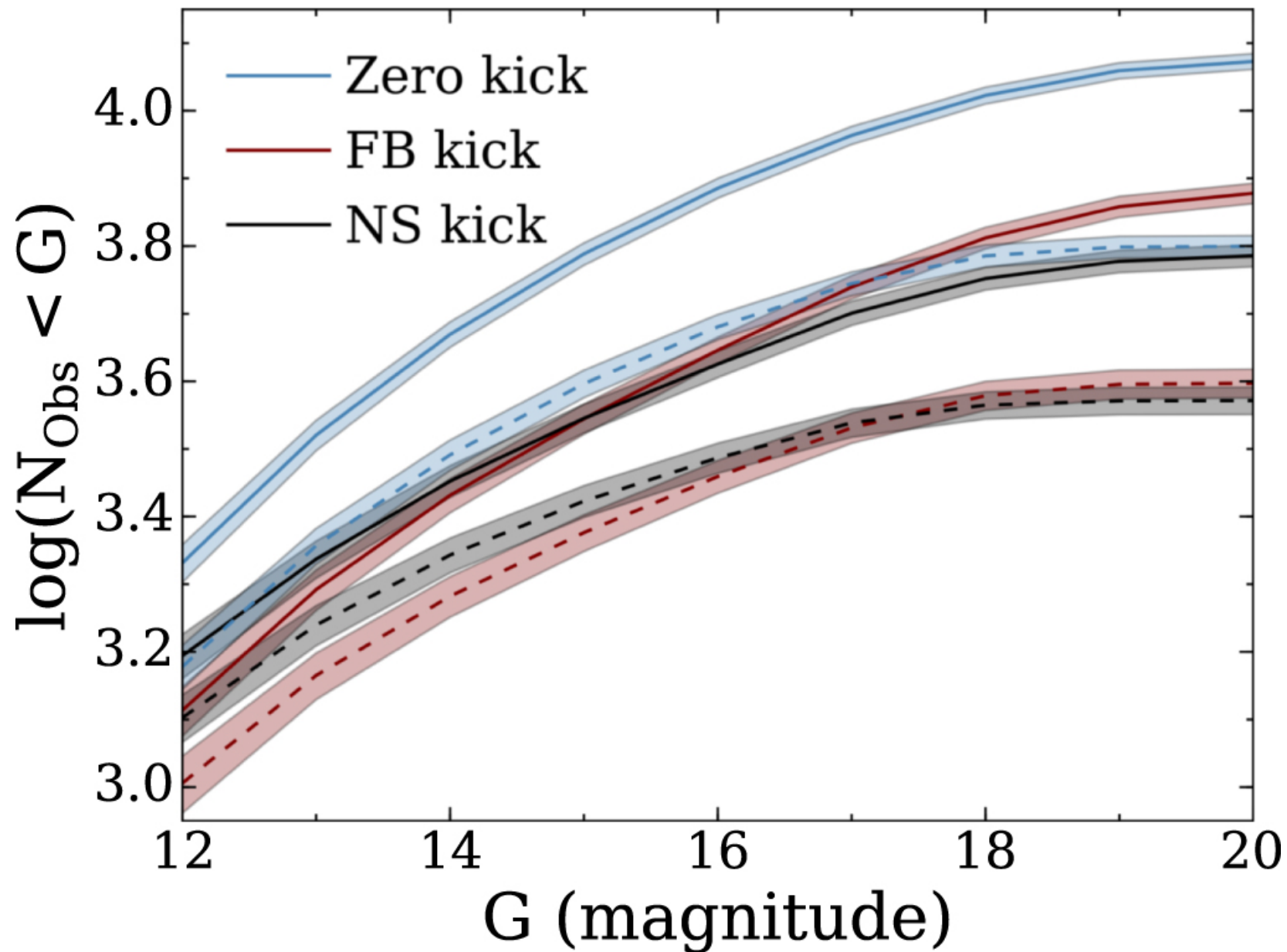
Figure 3. from Revealing Black Holes with Gaia null 2017 APJL 850 L13 doi:10.3847/2041-8213/aa97d5 https://dx.doi.org/10.3847/2041-8213/aa97d5 © 2017. The American Astronomical Society. All rights reserved.
