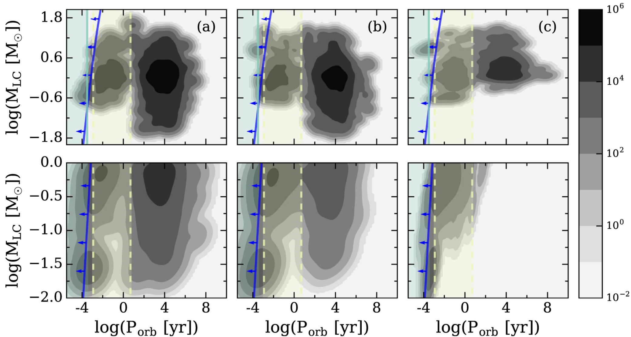
Figure 2. from Revealing Black Holes with Gaia null 2017 APJL 850 L13 doi:10.3847/2041-8213/aa97d5 https://dx.doi.org/10.3847/2041-8213/aa97d5 © 2017. The American Astronomical Society. All rights reserved.
