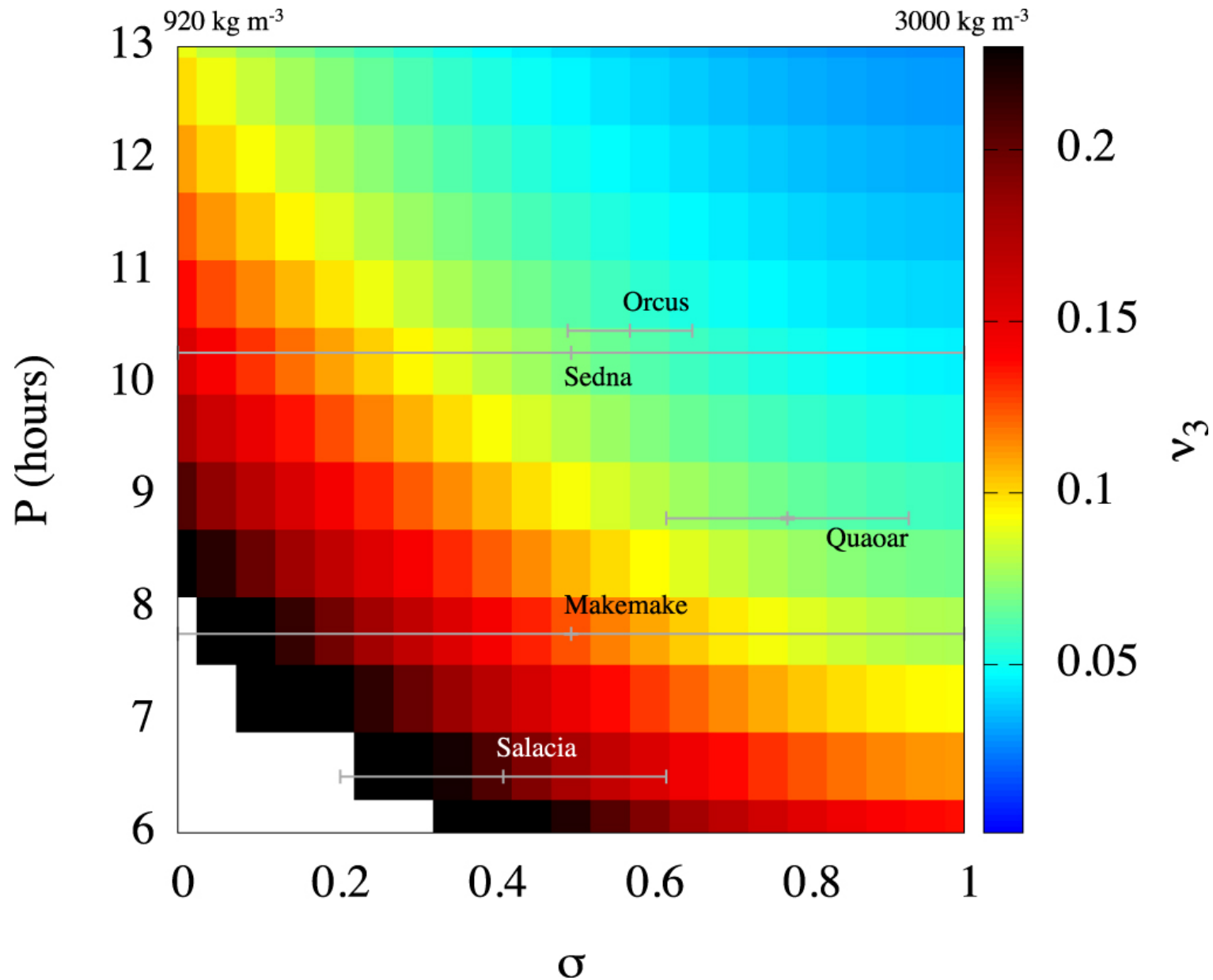
Figure 3. from Equilibrium Shapes of Large Trans-Neptunian Objects null 2017 APJL 850 L9 doi:10.3847/2041-8213/aa95bd https://dx.doi.org/10.3847/2041-8213/aa95bd © 2017. The American Astronomical Society. All rights reserved.
