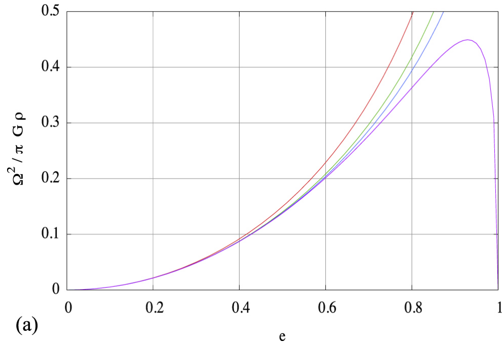
Figure 1. from Equilibrium Shapes of Large Trans-Neptunian Objects null 2017 APJL 850 L9 doi:10.3847/2041-8213/aa95bd https://dx.doi.org/10.3847/2041-8213/aa95bd © 2017. The American Astronomical Society. All rights reserved.
