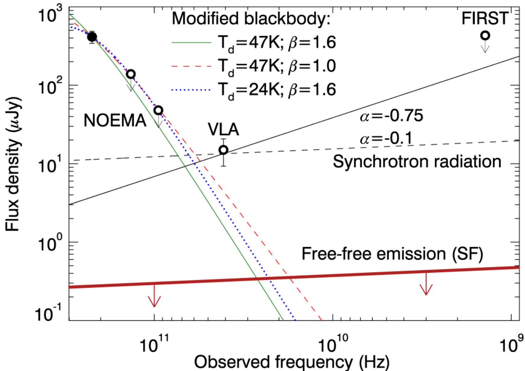
Figure 3. from Copious Amounts of Dust and Gas in a z = 7.5 Quasar Host Galaxy null 2017 APJL 851 L8 doi:10.3847/2041-8213/aa943a https://dx.doi.org/10.3847/2041-8213/aa943a © 2017. The American Astronomical Society. All rights reserved.
