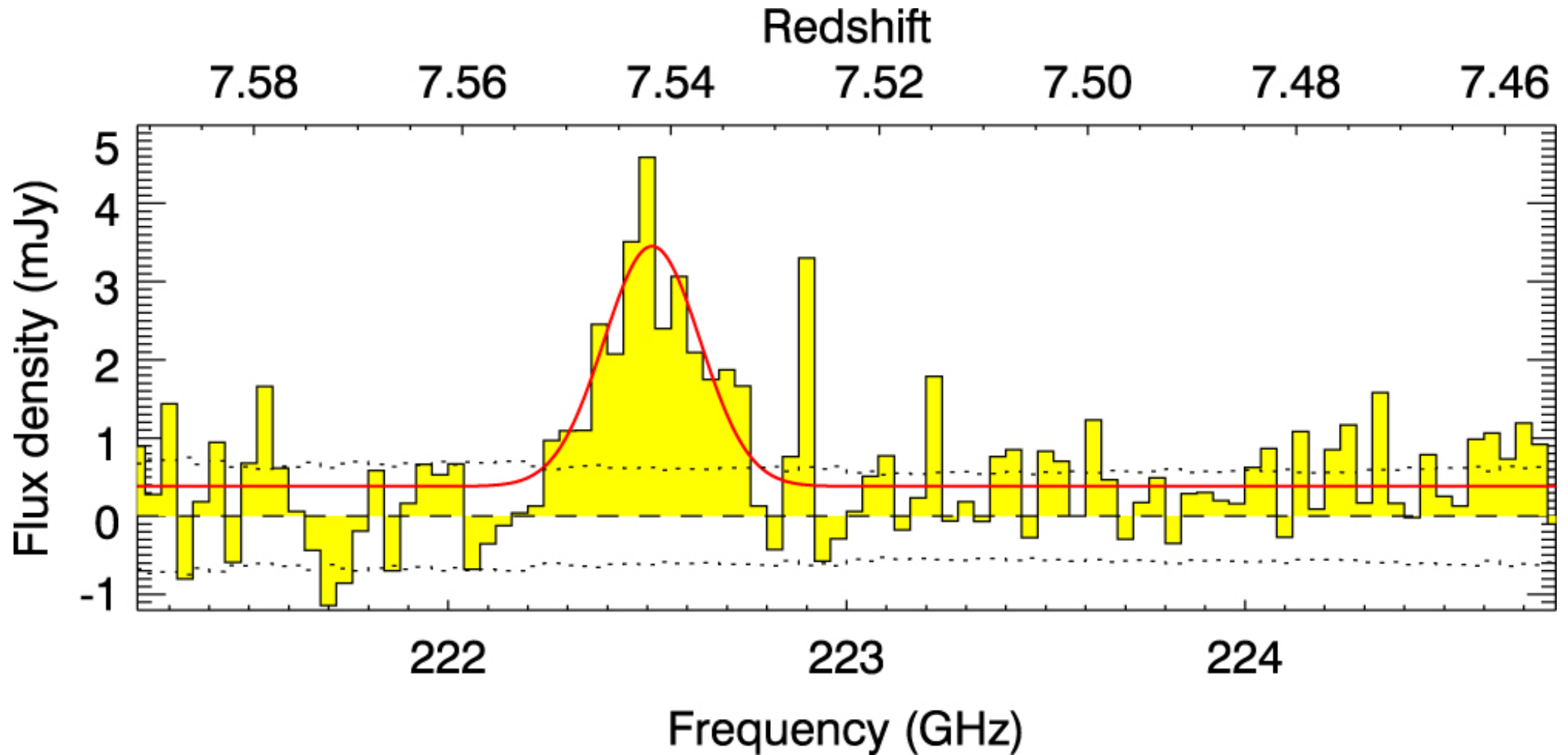
Figure 1. from Copious Amounts of Dust and Gas in a z = 7.5 Quasar Host Galaxy null 2017 APJL 851 L8 doi:10.3847/2041-8213/aa943a https://dx.doi.org/10.3847/2041-8213/aa943a © 2017. The American Astronomical Society. All rights reserved.
