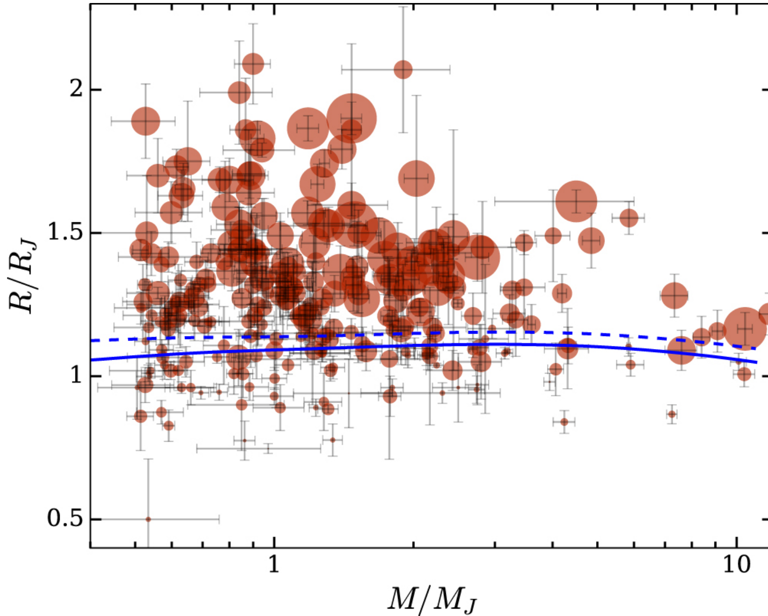
Figure 1. from Estimating the Magnetic Field Strength in Hot Jupiters null 2017 APJL 849 L12 doi:10.3847/2041-8213/aa93fd https://dx.doi.org/10.3847/2041-8213/aa93fd © 2017. The American Astronomical Society. All rights reserved.
