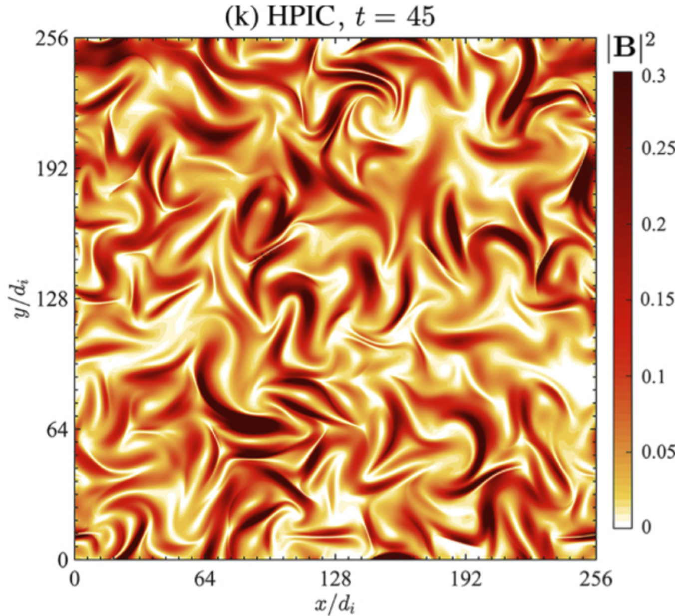
Figure 2. from Magnetic Reconnection as a Driver for a Sub-ion-scale Cascade in Plasma Turbulence null 2017 APJL 850 L16 doi:10.3847/2041-8213/aa93fb https://dx.doi.org/10.3847/2041-8213/aa93fb © 2017. The American Astronomical Society. All rights reserved.
