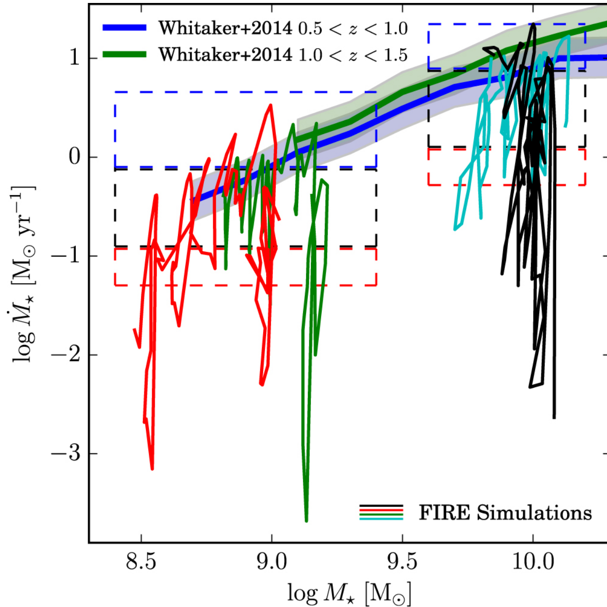
Figure 2. from Stacked Star Formation Rate Profiles of Bursty Galaxies Exhibit “Coherent” Star Formation null 2017 APJL 849 L2 doi:10.3847/2041-8213/aa8f93 https://dx.doi.org/10.3847/2041-8213/aa8f93 © 2017. The American Astronomical Society. All rights reserved.
