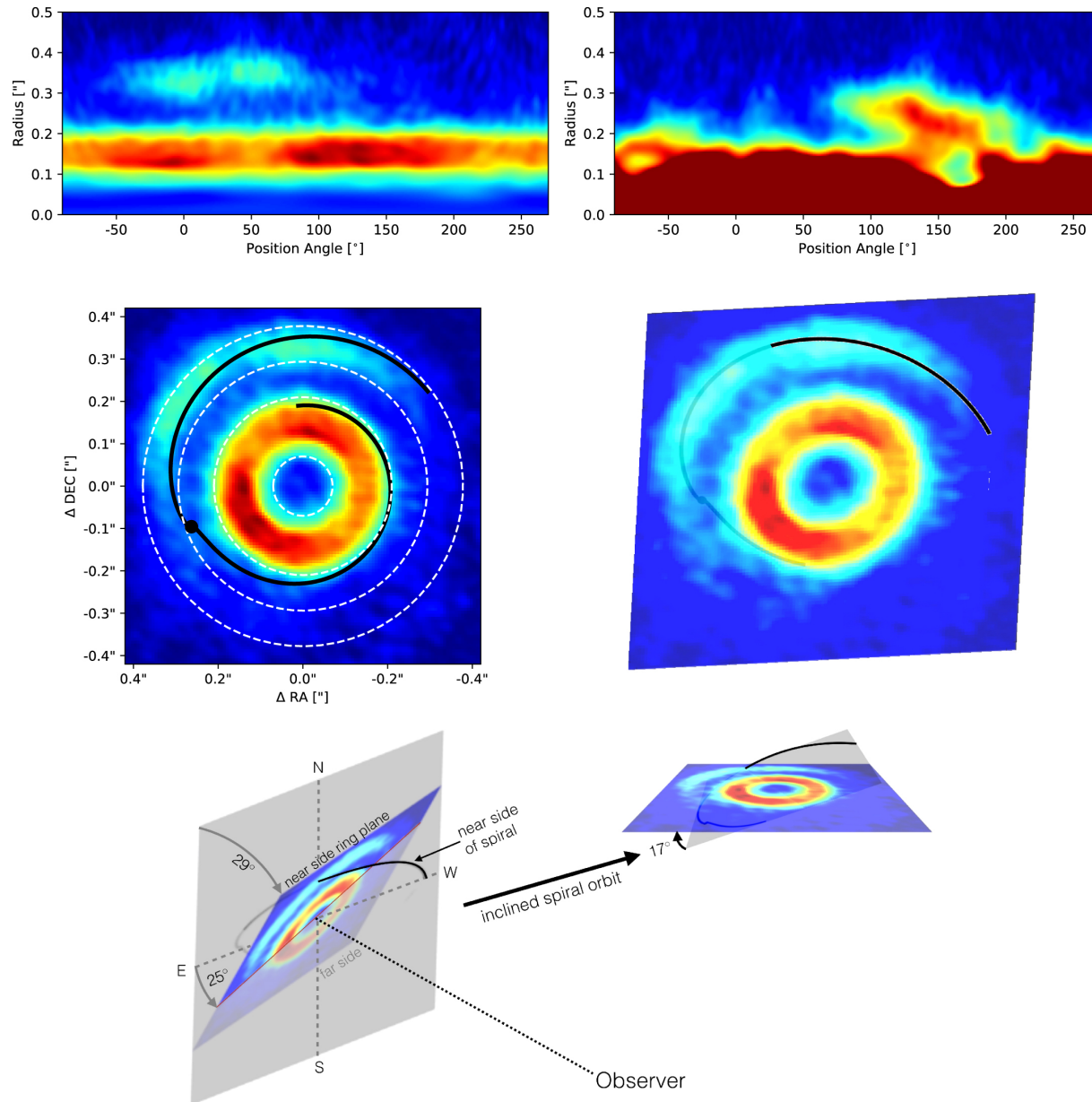
Figure 3. from Dust-trapping Vortices and a Potentially Planet-triggered Spiral Wake in the Pre-transitional Disk of V1247 Orionis null 2017 APJL 848 L11 doi:10.3847/2041-8213/aa8edc https://dx.doi.org/10.3847/2041-8213/aa8edc
