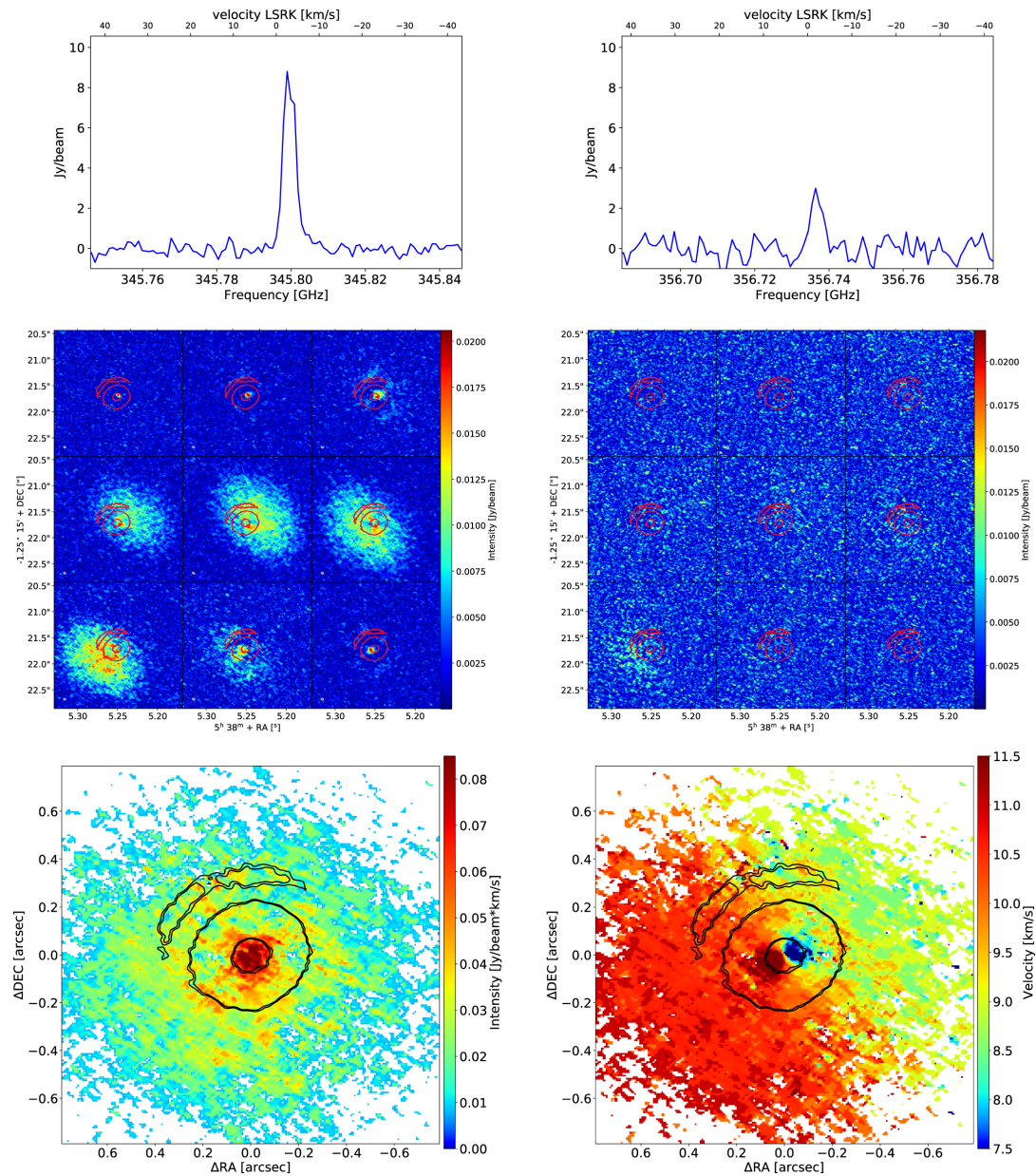
Figure 2. from Dust-trapping Vortices and a Potentially Planet-triggered Spiral Wake in the Pre-transitional Disk of V1247 Orionis null 2017 APJL 848 L11 doi:10.3847/2041-8213/aa8edc https://dx.doi.org/10.3847/2041-8213/aa8edc © 2017. The American Astronomical Society. All rights reserved.
