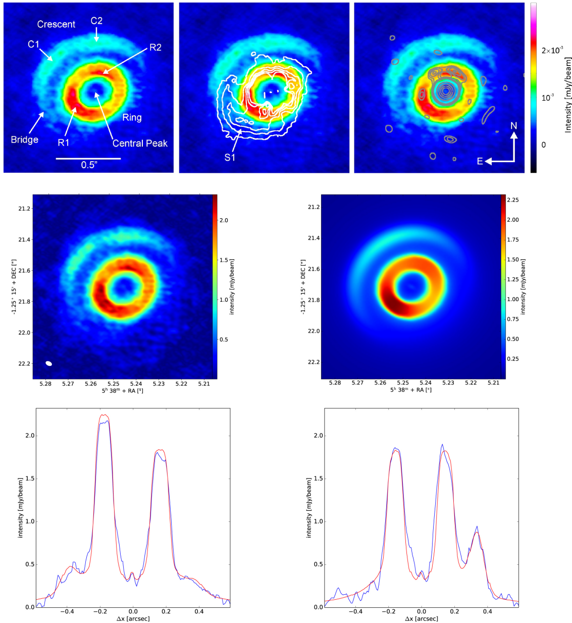
Figure 1. from Dust-trapping Vortices and a Potentially Planet-triggered Spiral Wake in the Pre-transitional Disk of V1247 Orionis null 2017 APJL 848 L11 doi:10.3847/2041-8213/aa8edc https://dx.doi.org/10.3847/2041-8213/aa8edc © 2017. The American Astronomical Society. All rights reserved.
