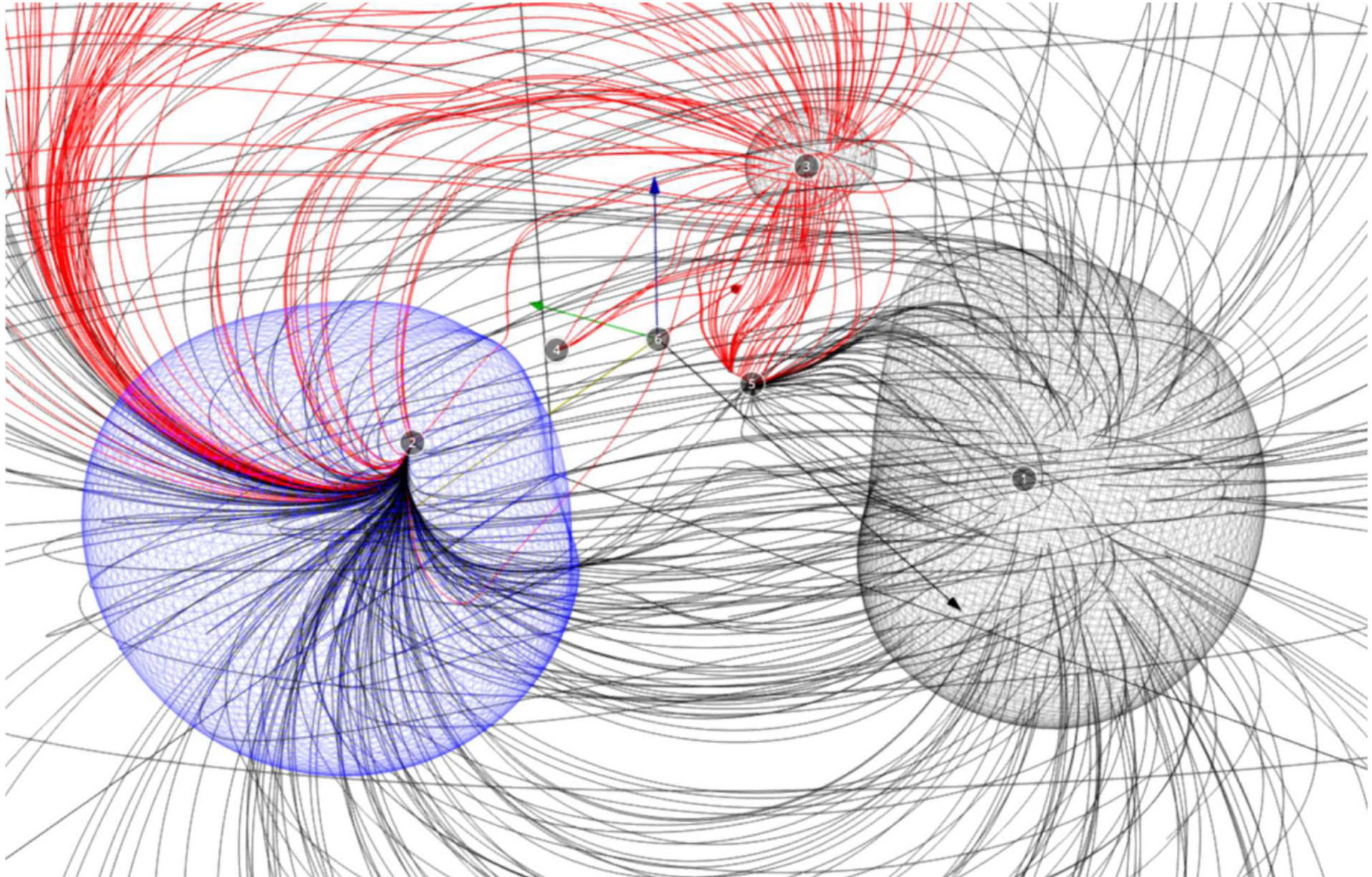
Figure 2. from Cosmicflows-3: Cold Spot Repeller? null 2017 APJL 847 L6 doi:10.3847/2041-8213/aa88b2 https://dx.doi.org/10.3847/2041-8213/aa88b2 © 2017. The American Astronomical Society. All rights reserved.
