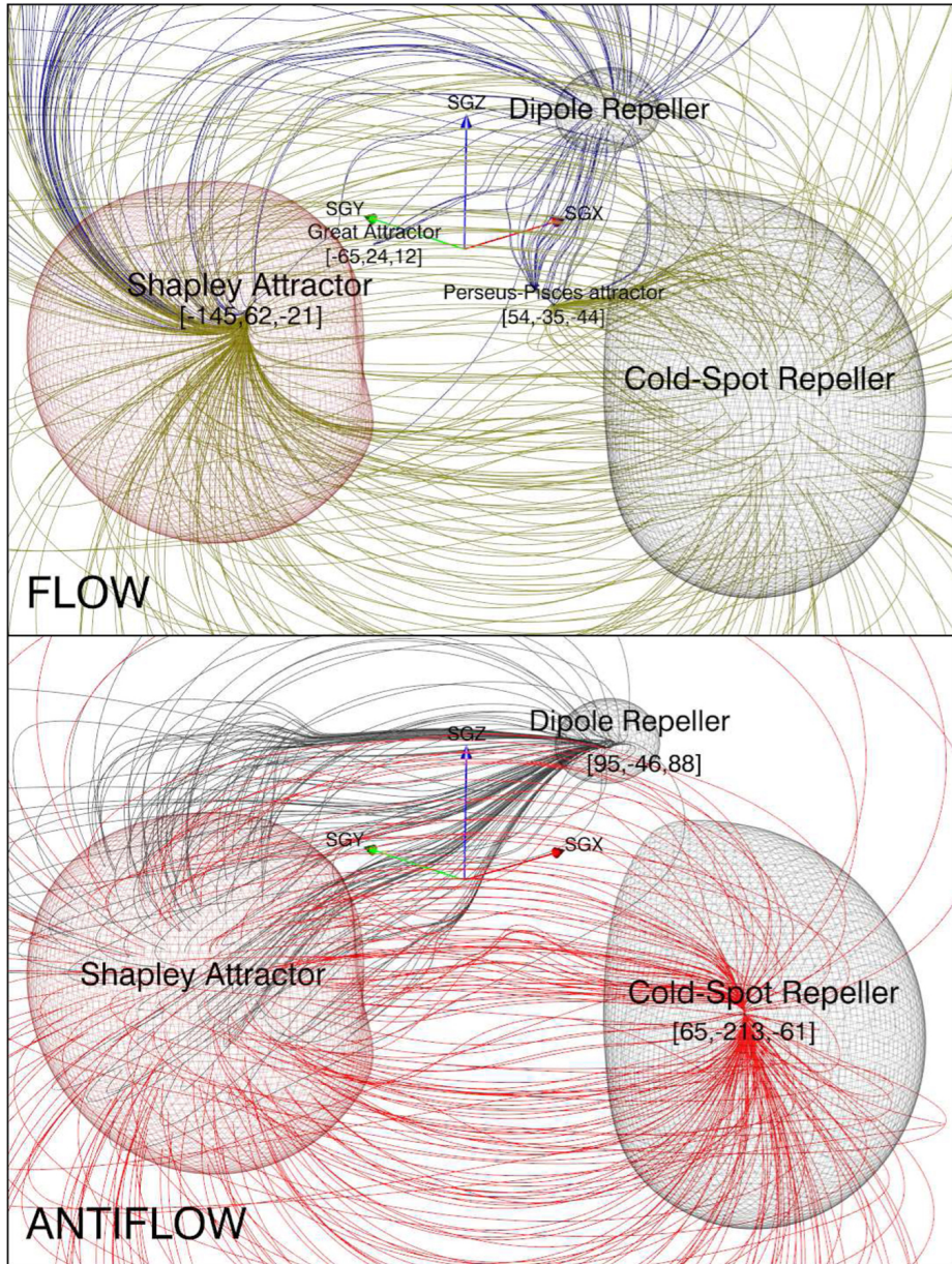
Figure 1. from Cosmicflows-3: Cold Spot Repeller? null 2017 APJL 847 L6 doi:10.3847/2041-8213/aa88b2 https://dx.doi.org/10.3847/2041-8213/aa88b2 © 2017. The American Astronomical Society. All rights reserved.
