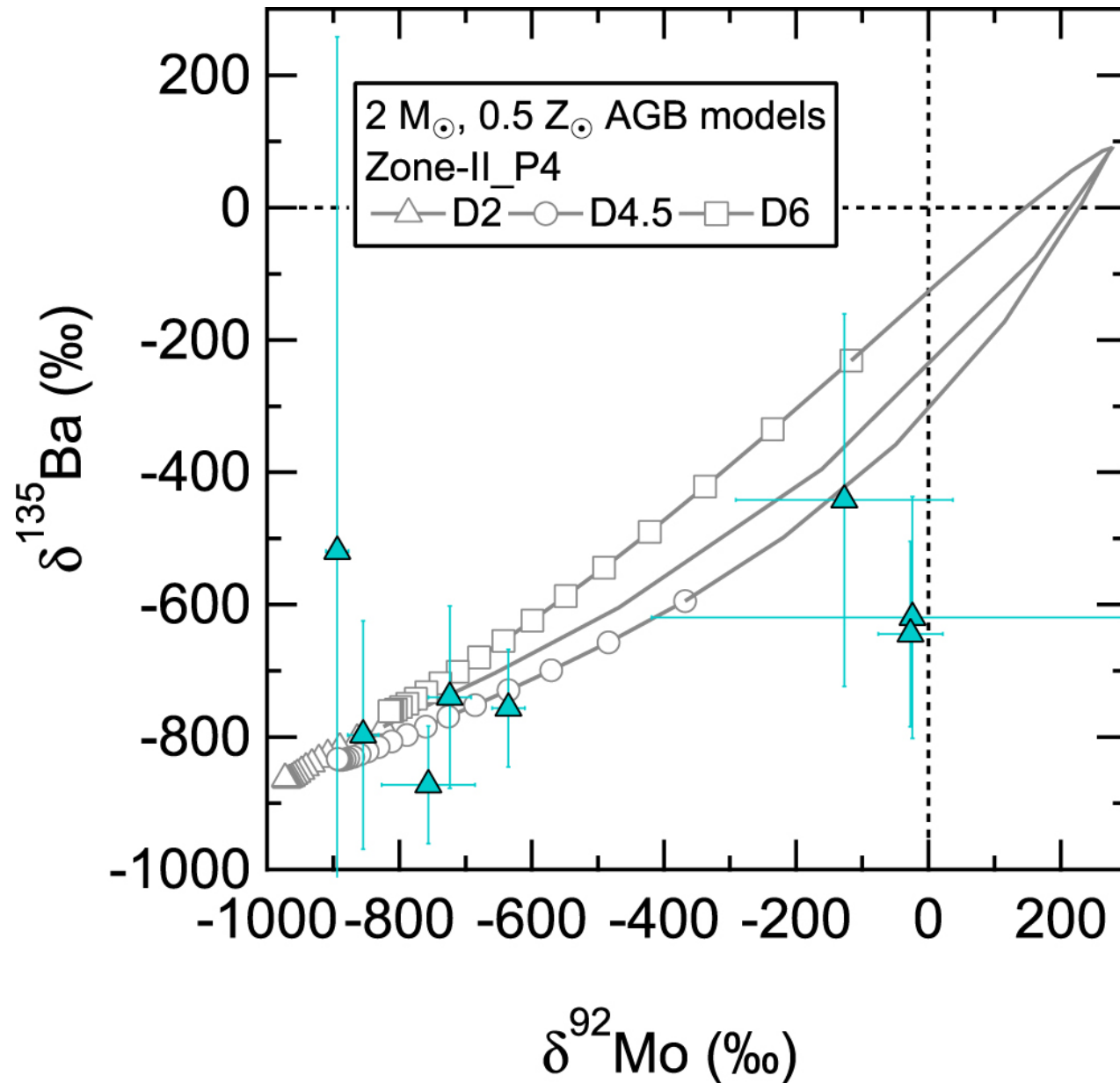
Figure 4. from J-type Carbon Stars: A Dominant Source of ^{14}\text{N} -rich Presolar SiC Grains of Type AB null 2017 APJL 844 L12 doi:10.3847/2041-8213/aa7d4c https://dx.doi.org/10.3847/2041-8213/aa7d4c © 2017. The American Astronomical Society. All rights reserved.
