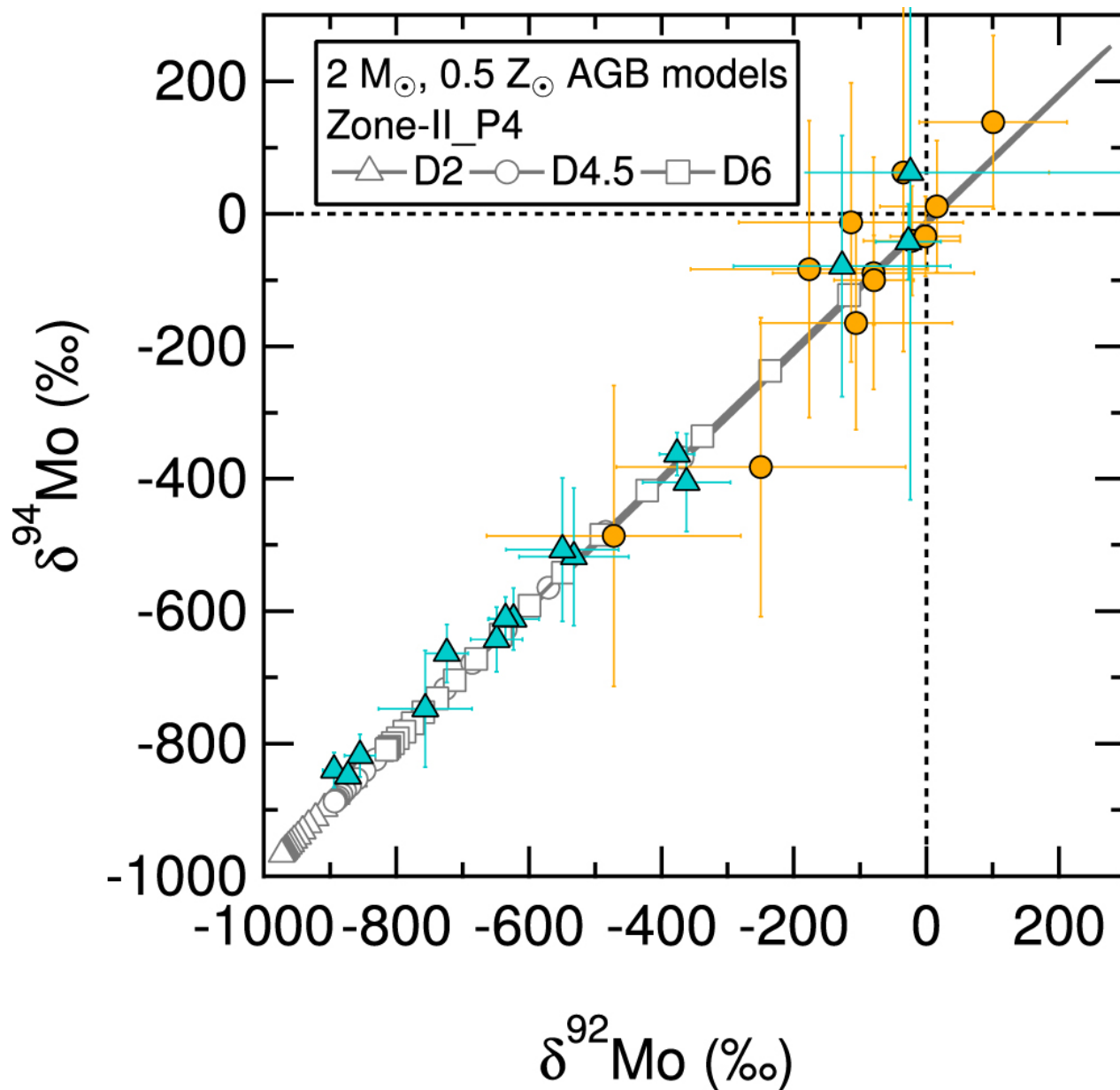
Figure 2. from J-type Carbon Stars: A Dominant Source of ^{14}\text{N} -rich Presolar SiC Grains of Type AB null 2017 APJL 844 L12 doi:10.3847/2041-8213/aa7d4c https://dx.doi.org/10.3847/2041-8213/aa7d4c © 2017. The American Astronomical Society. All rights reserved.
