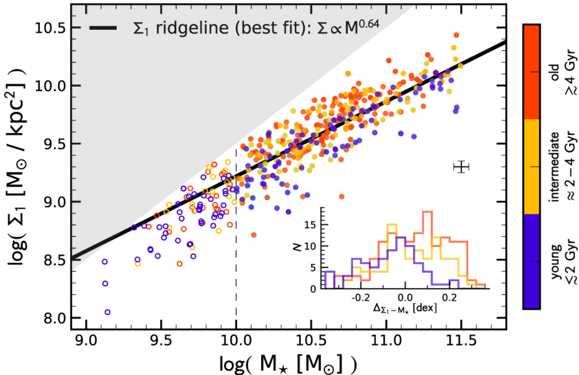
Figure 4. from On the Evolution of the Central Density of Quiescent Galaxies null 2017 APJL 844 L1 doi:10.3847/2041-8213/aa7cfb https://dx.doi.org/10.3847/2041-8213/aa7cfb © 2017. The American Astronomical Society. All rights reserved.
