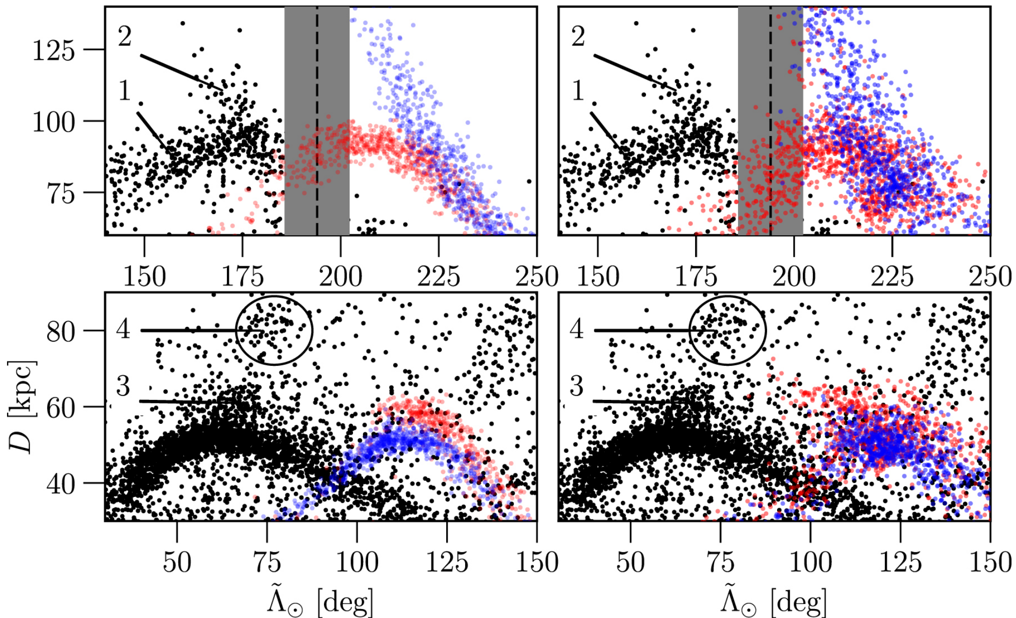
Figure 4. from The >100 kpc Distant Spur of the Sagittarius Stream and the Outer Virgo Overdensity, as Seen in PS1 RR Lyrae Stars null 2017 APJL 844 L4 doi:10.3847/2041-8213/aa7c61 https://dx.doi.org/10.3847/2041-8213/aa7c61 © 2017. The American Astronomical Society. All rights reserved.
