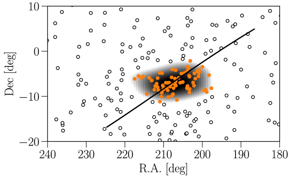
Figure 3. from The >100 kpc Distant Spur of the Sagittarius Stream and the Outer Virgo Overdensity, as Seen in PS1 RR Lyrae Stars null 2017 APJL 844 L4 doi:10.3847/2041-8213/aa7c61 https://dx.doi.org/10.3847/2041-8213/aa7c61 © 2017. The American Astronomical Society. All rights reserved.
