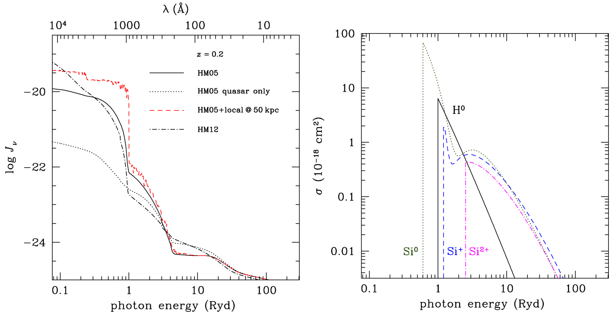
Figure 1. from Gauging Metallicity of Diffuse Gas under an Uncertain Ionizing Radiation Field null 2017 APJL 842 L19 doi:10.3847/2041-8213/aa762d https://dx.doi.org/10.3847/2041-8213/aa762d © 2017. The American Astronomical Society. All rights reserved.
